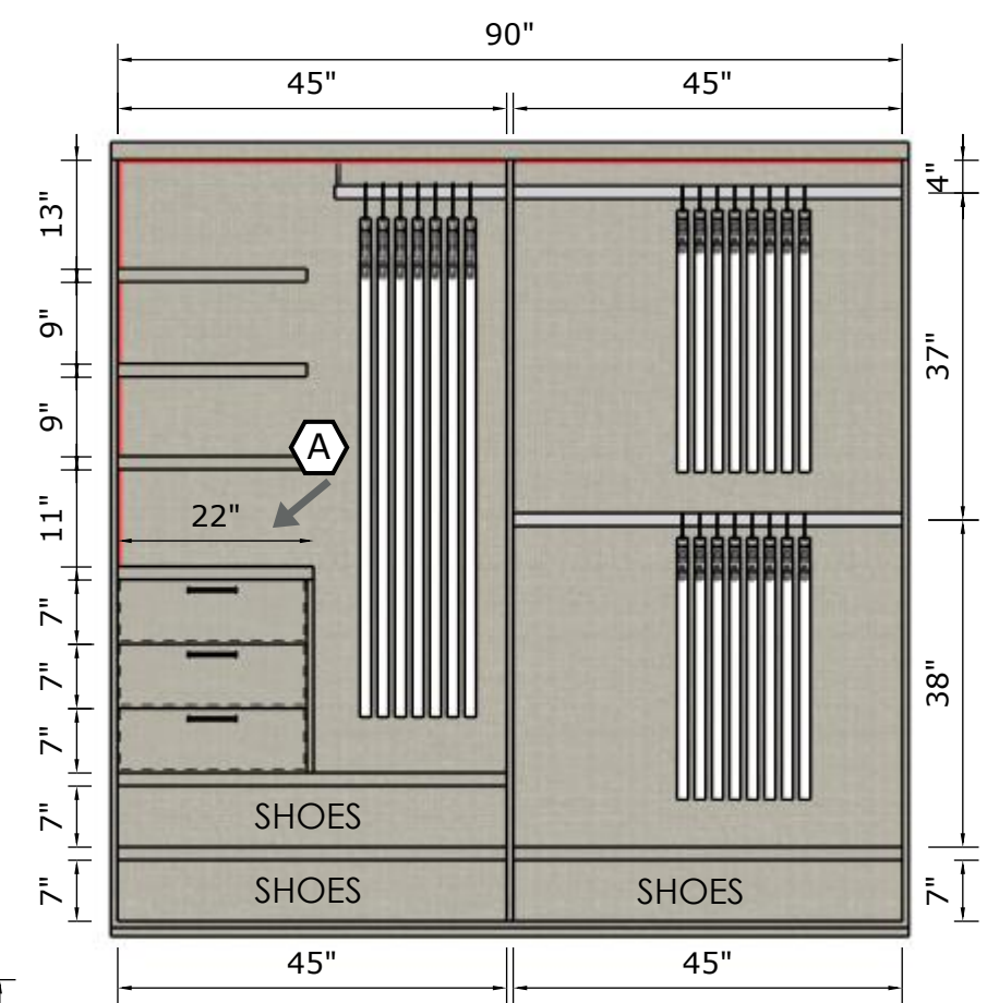
FRONT VIEW Scale 1:24
