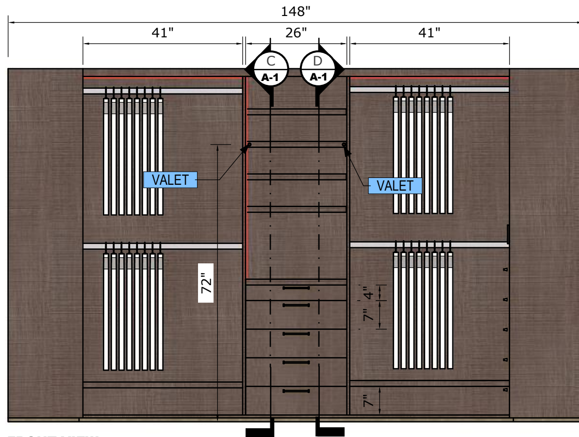
FRONT VIEW Scale 1:24
