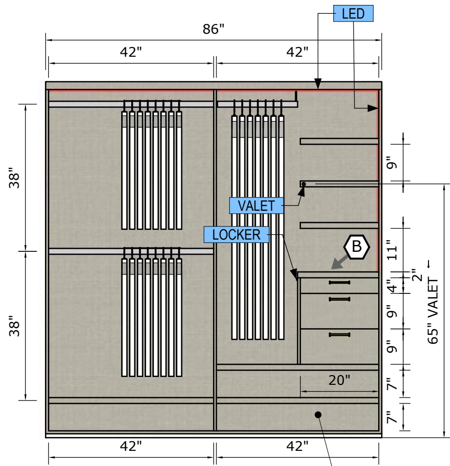
FRONT VIEW Scale 1:24
