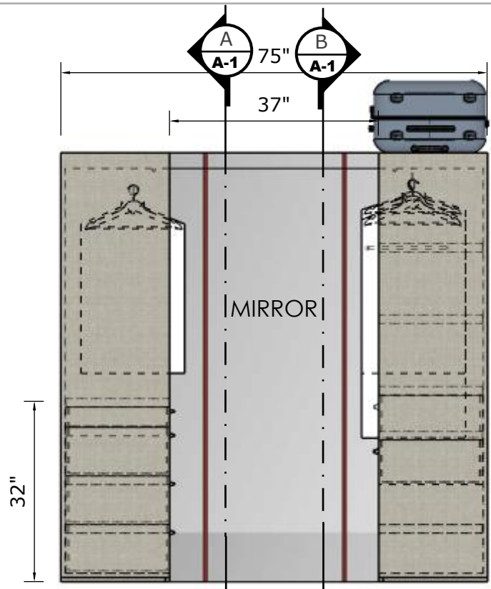
FRONT VIEW Scale 1:24
