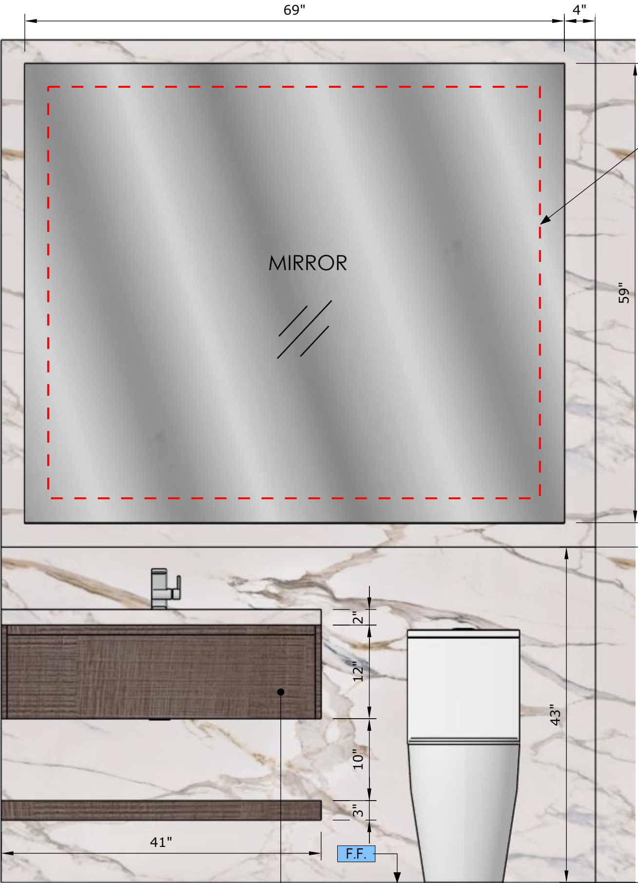
FRONT VIEW Scale 1:12
