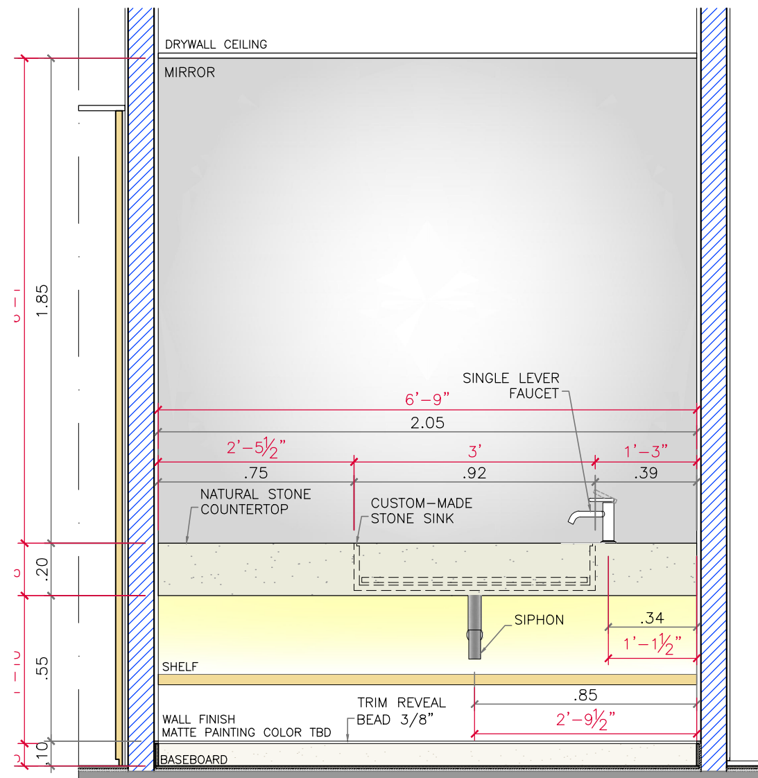
ELEVATION 01 scale 1:25
