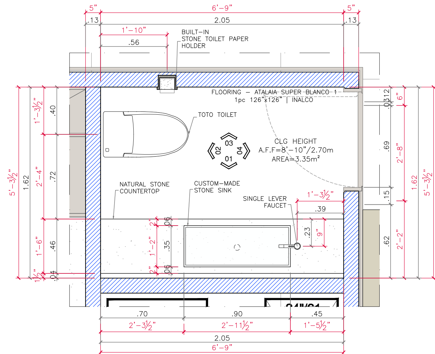
PLAN scale 1:25 | scale: 1/2" = 1'-0"
