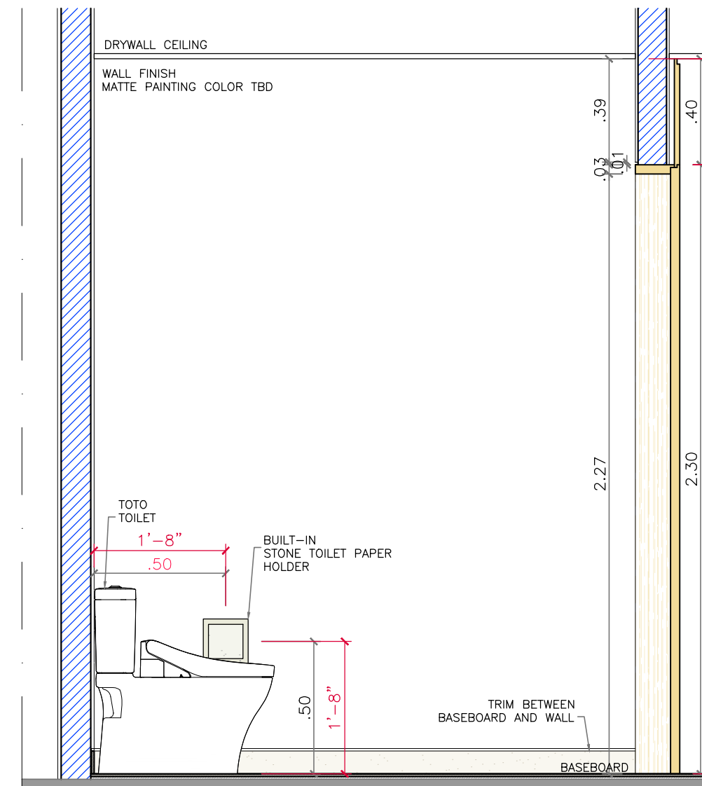
ELEVATION 03 scale 1:25
