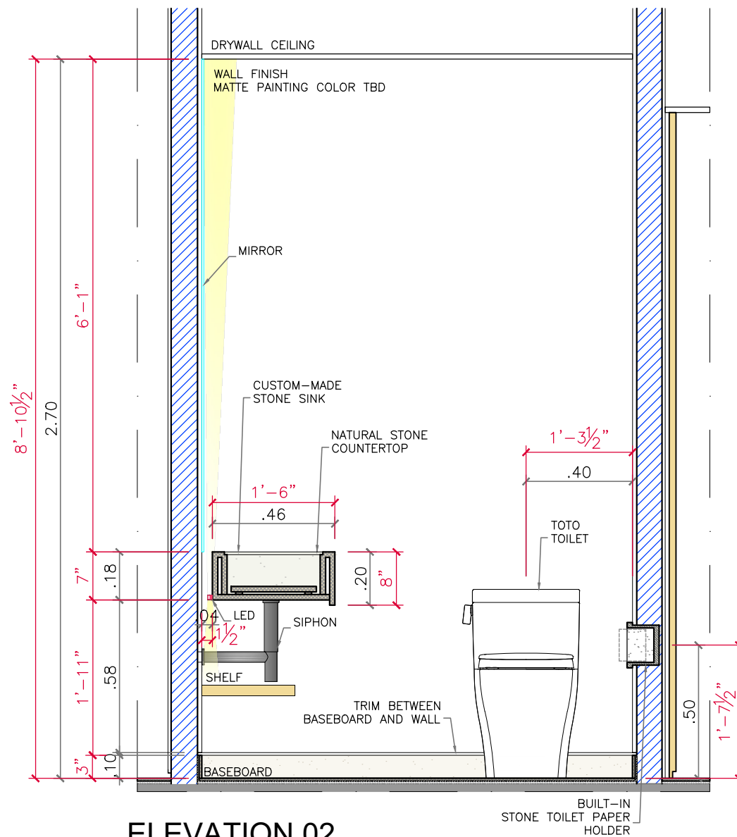
ELEVATION 02 scale 1:25
