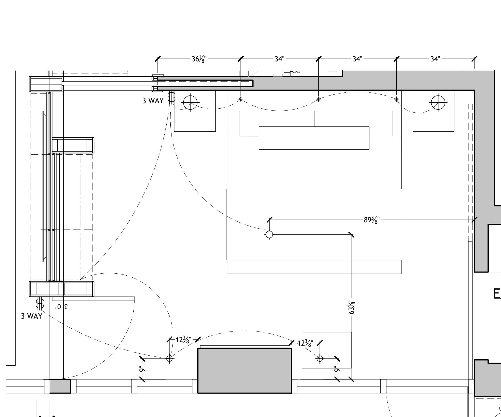
2 RCP & LIGHTING PLAN 103.2 SCALE 1/2"=1'-0"
