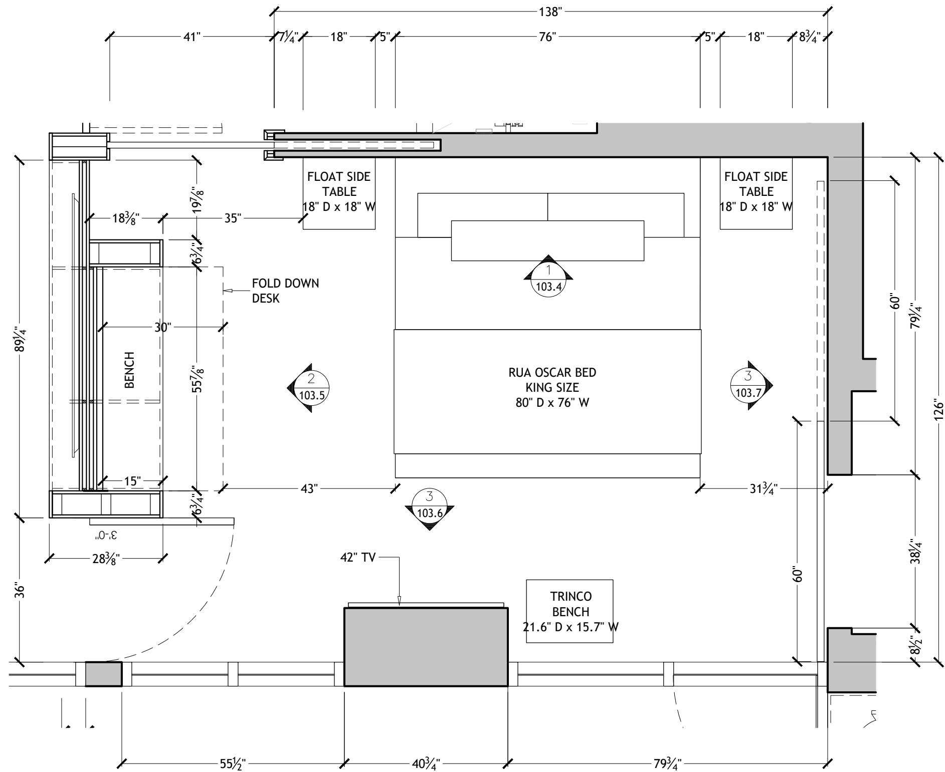
1 PLAN 103.1 SCALE 1/2"=1'-0"
