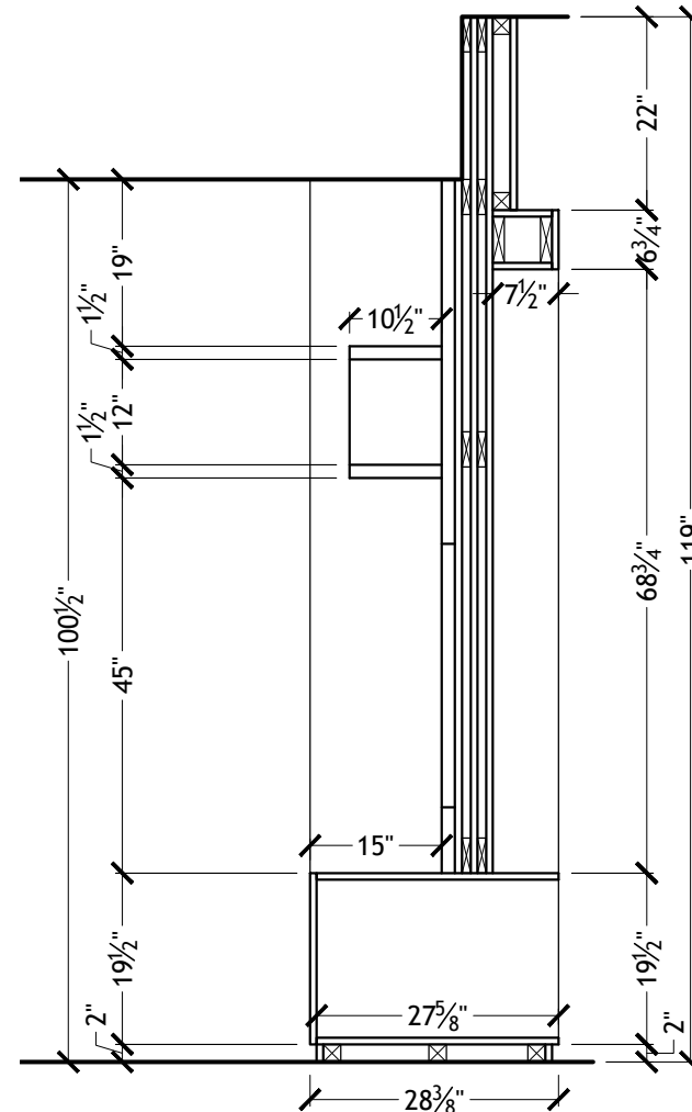
3 SECTION 103.5 SCALE 1/2"=1'-0"
