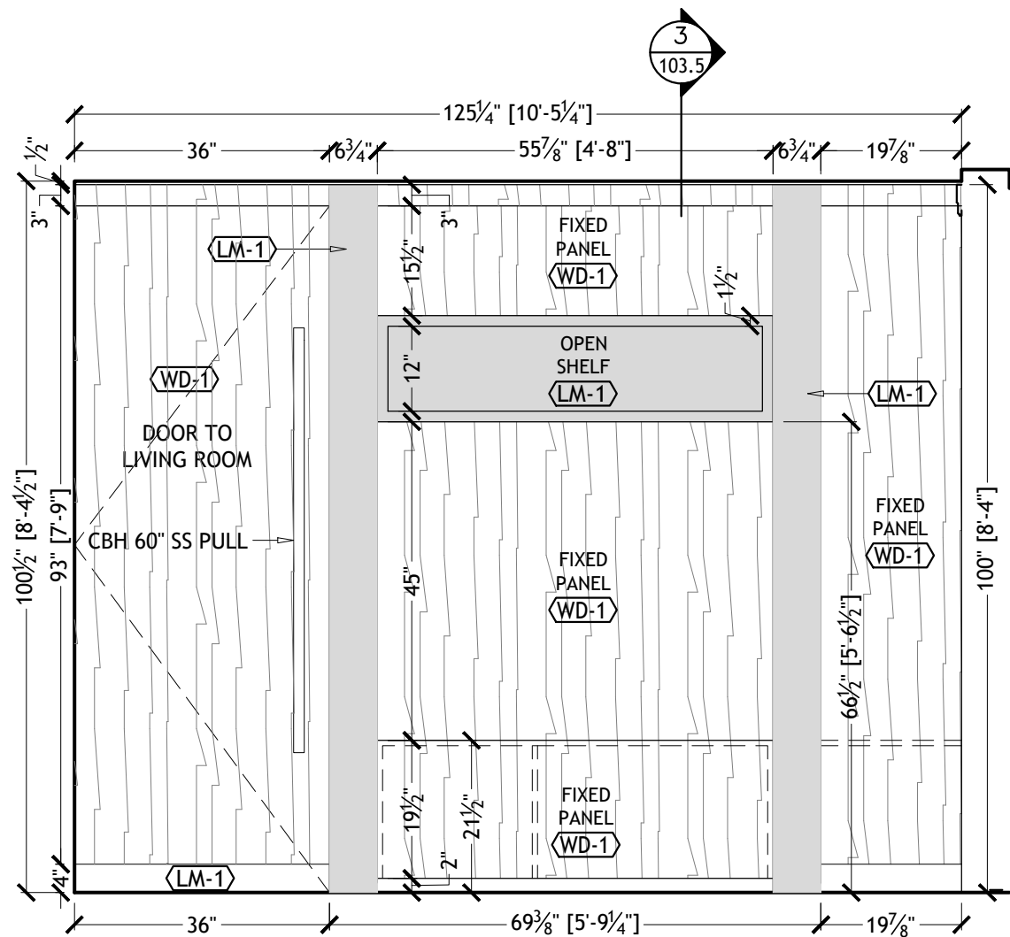
2 ELEVATION 104.5 SCALE 1/2"=1'-0"
