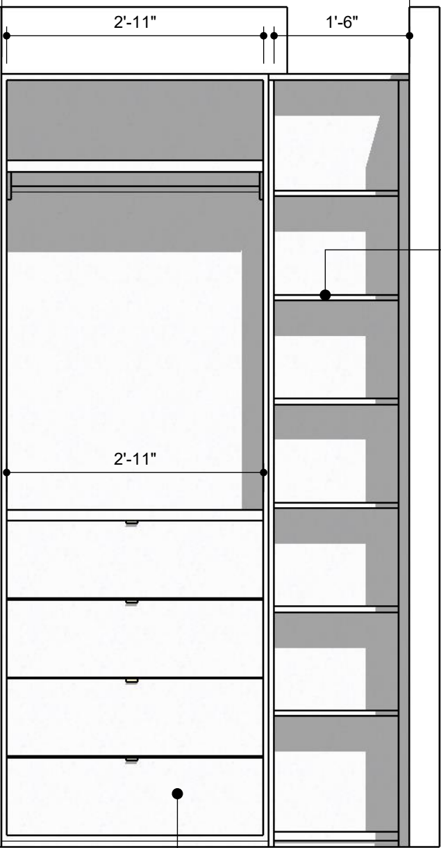
FRONT VIEW Scale 1:8
