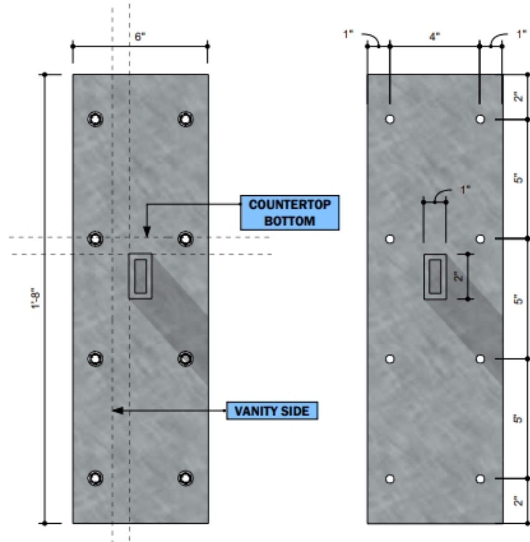
FRONT VIEW Scale 1:4
