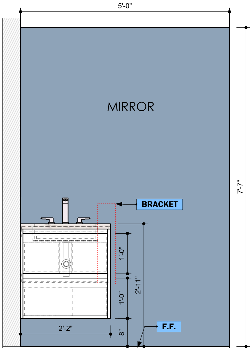
FRONT VIEW Scale 1:16
