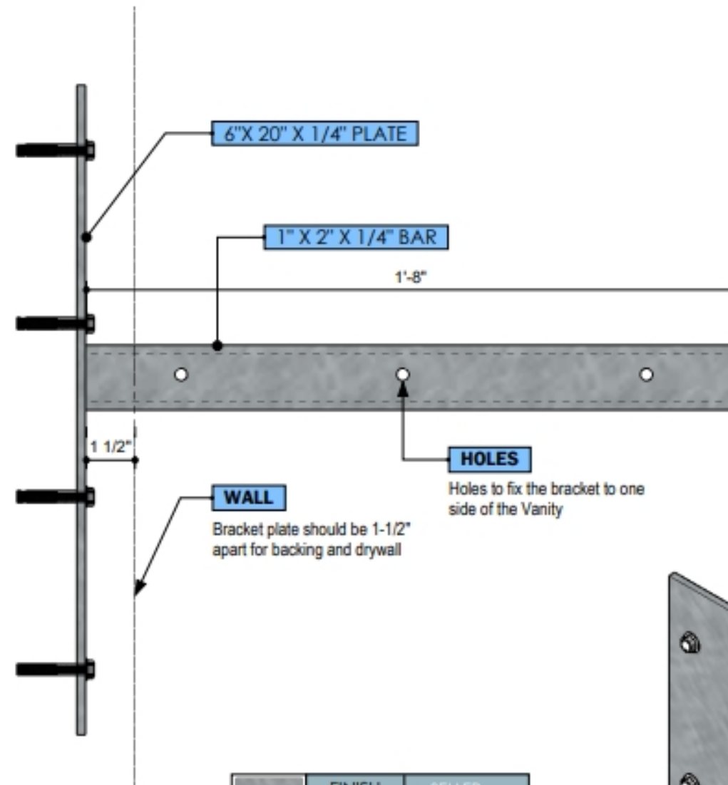
SIDE VIEW Scale 1:4
