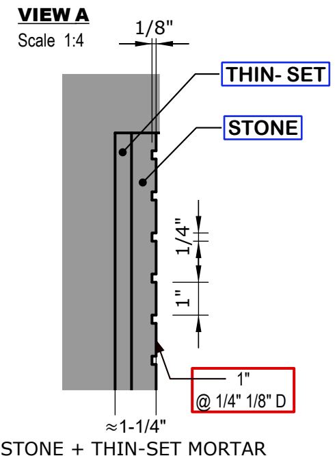
STONE + THIN-SET MORTAR
