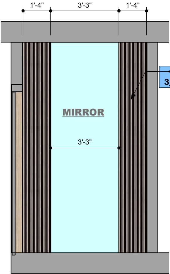
VIEW (2) Scale 1:32
