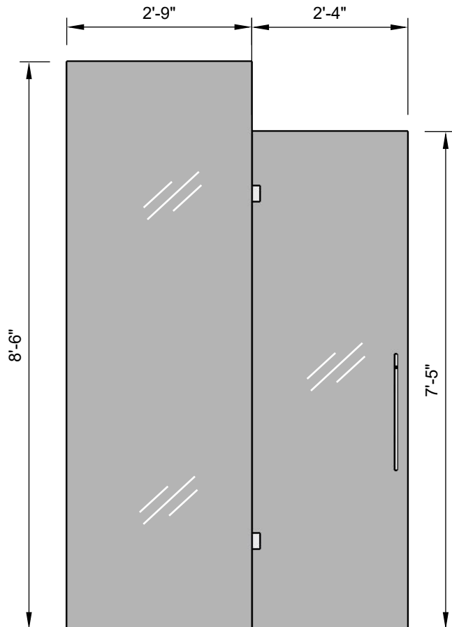
BATHROOM No 2 Scale 1:24
