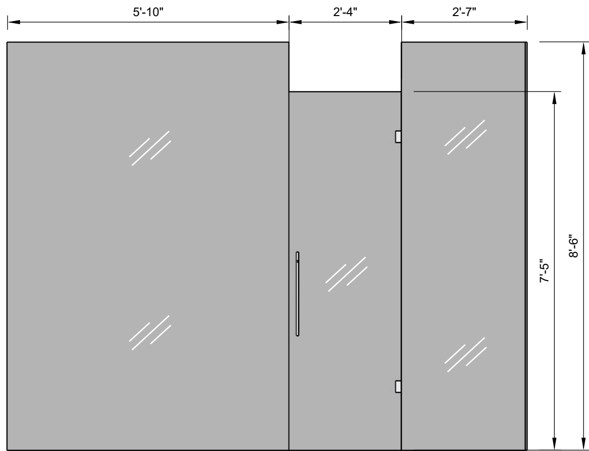
MASTER BATHROOM FRONT VIEW Scale 1:24
