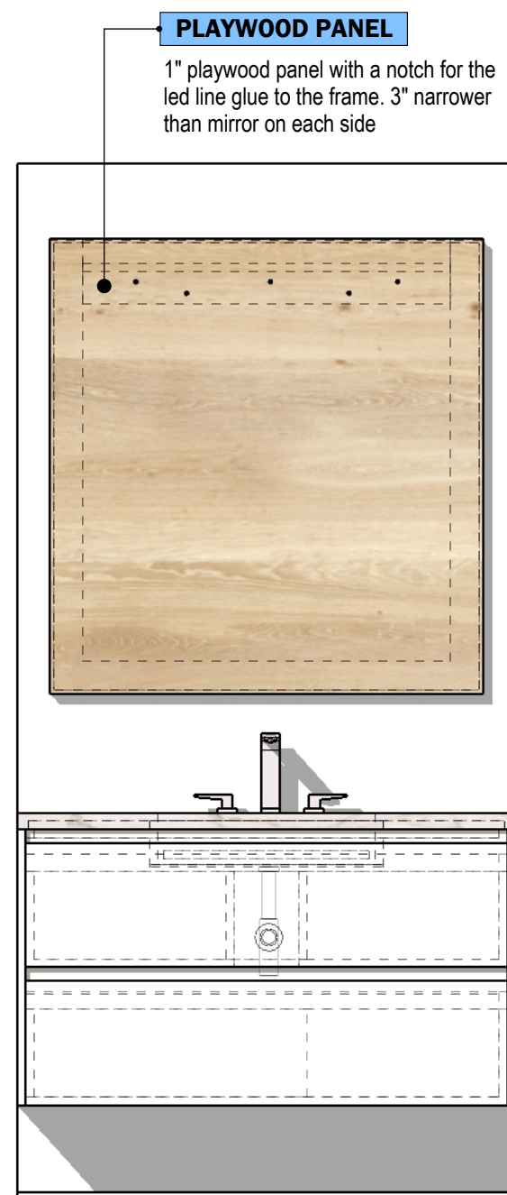
C FRONT VIEW Scale 1:16
