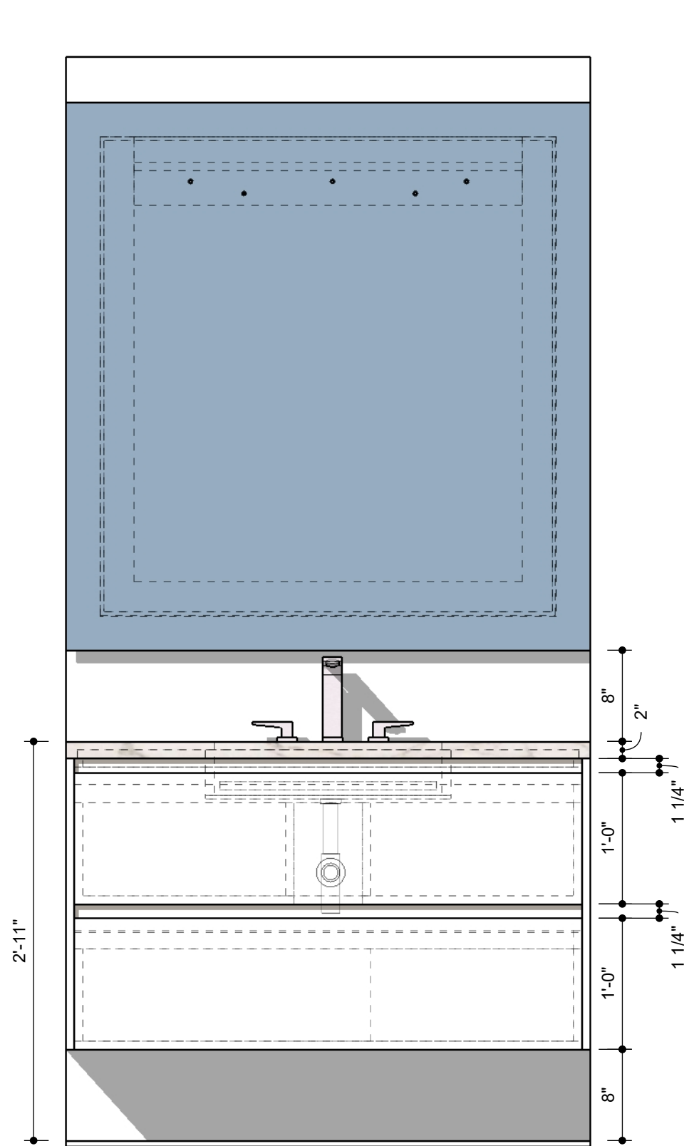
FRONT VIEW Scale 1:12
