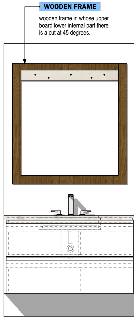
B FRONT VIEW Scale 1:16
