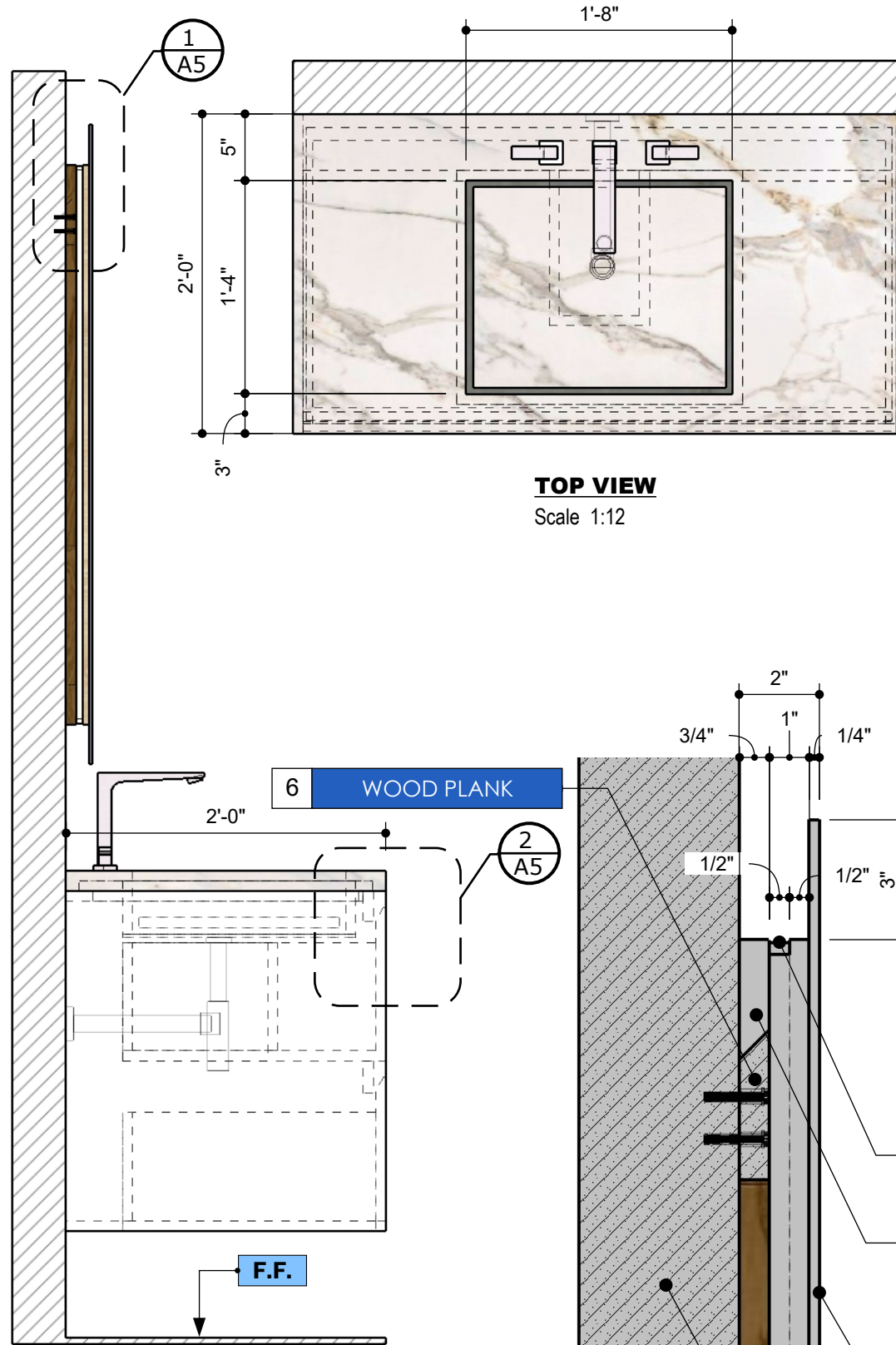
SIDE VIEW Scale 1:12
