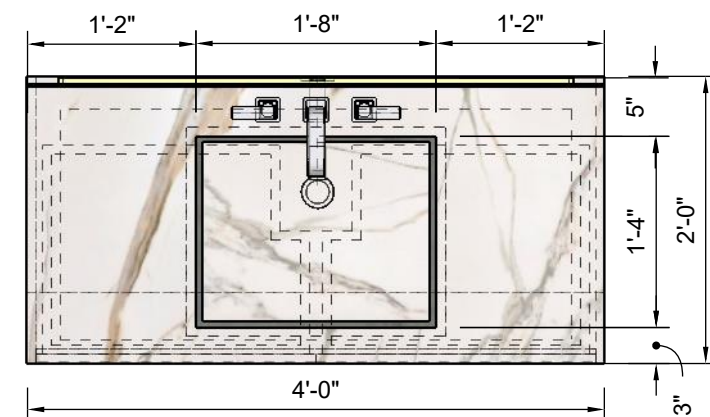
TOP VIEW Scale 1:16
