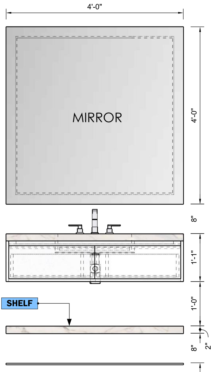
FRONT VIEW Scale 1:16
