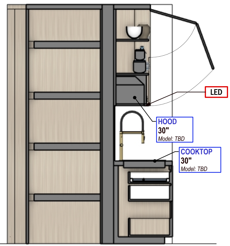
SECTION C Scale 1:24
