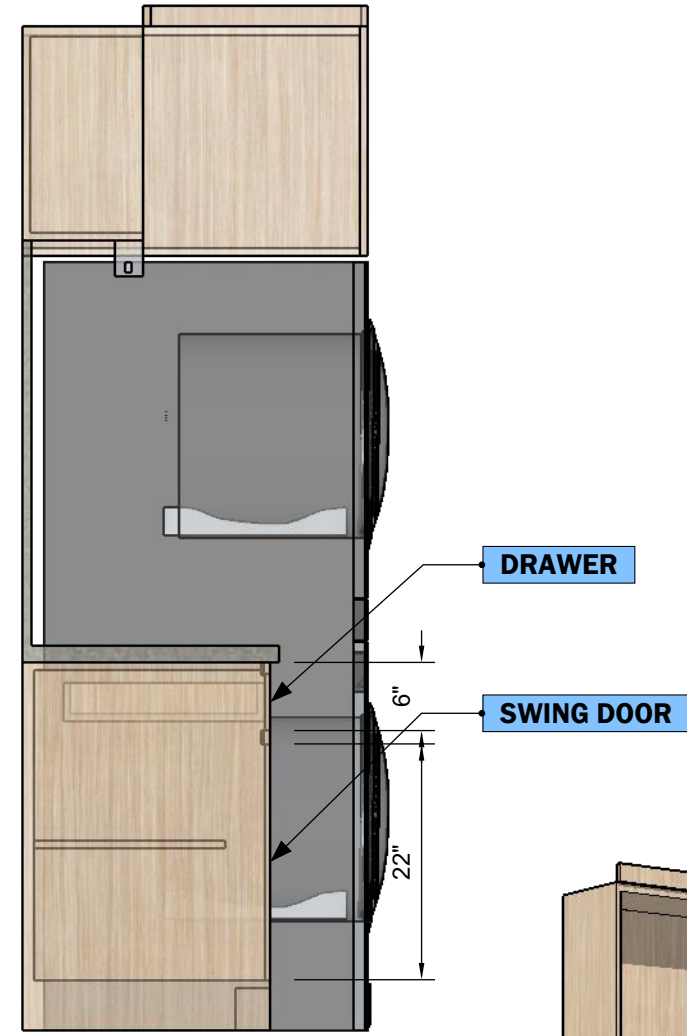
SIDE VIEW Scale 1:18
