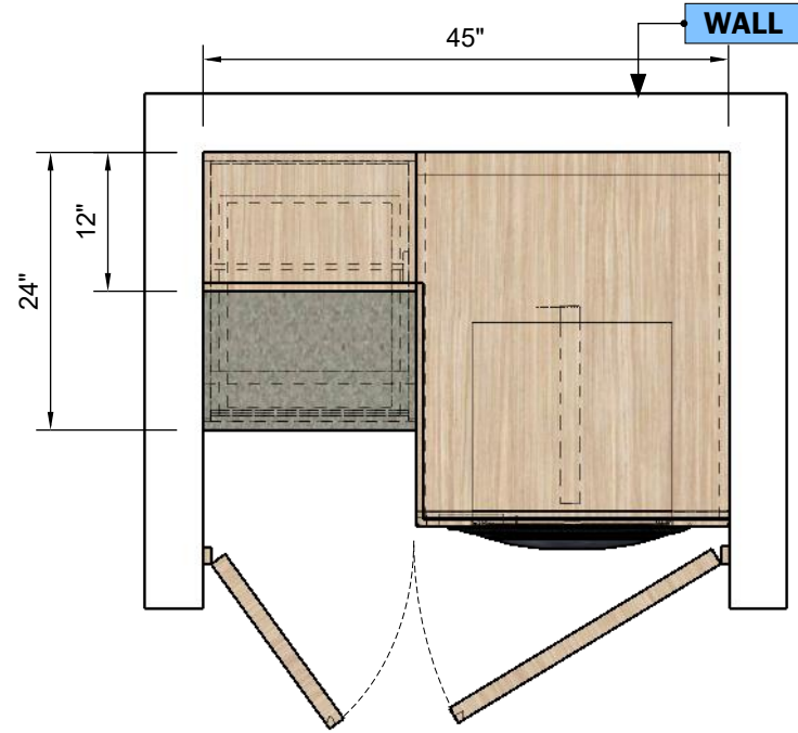
TOP VIEW Scale 1:18
