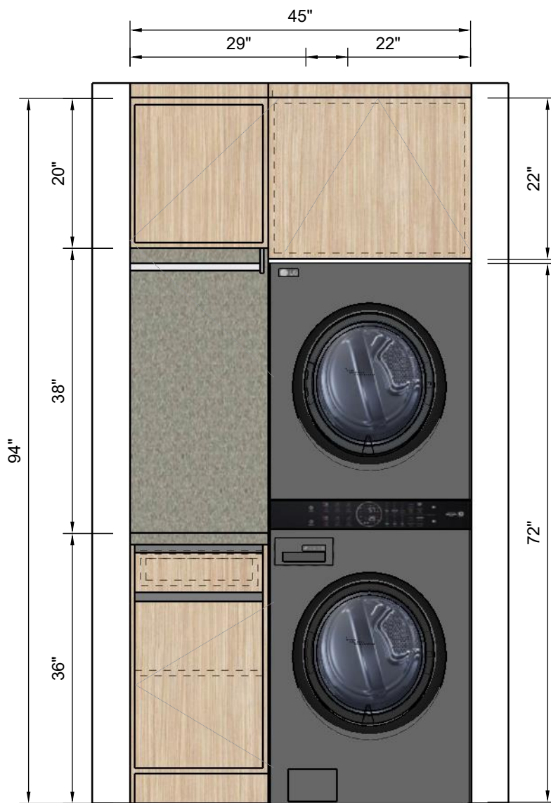
FRONT VIEW Scale 1:18
