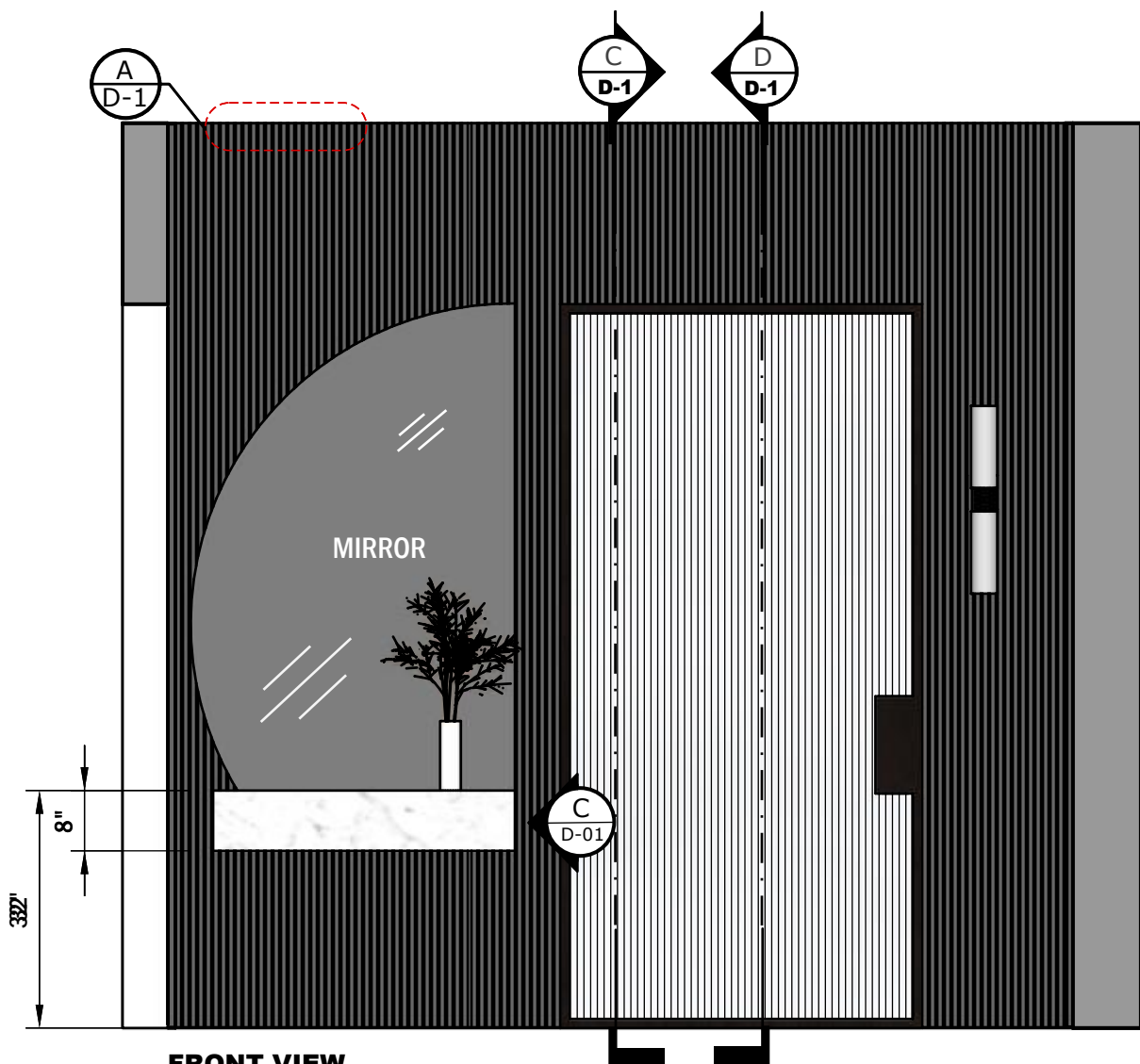
FRONT VIEW Scale 1:24
