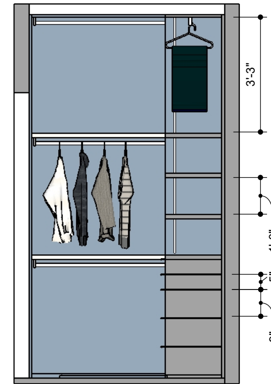
VIEW 5 Scale 1:32
