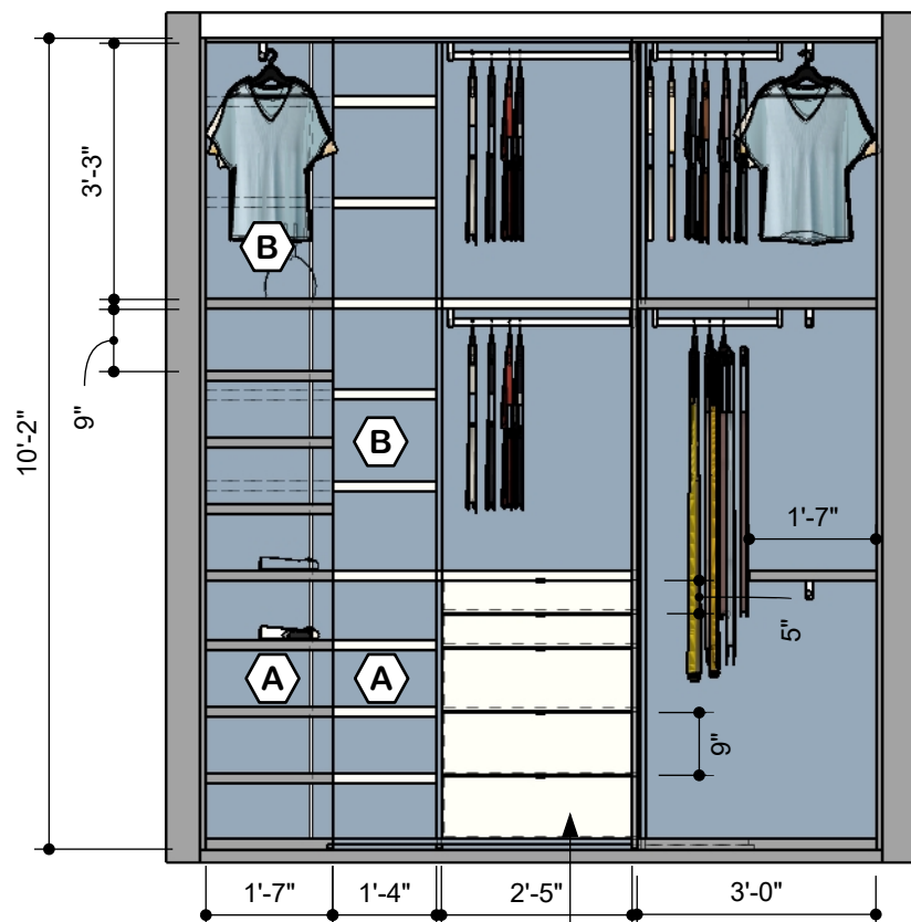
JUNIOR CLOSET FRONT VIEW Scale 1:32
