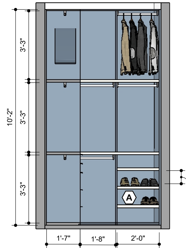
VIEW 6 Scale 1:32
