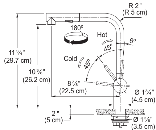
Dimensional Drawing
