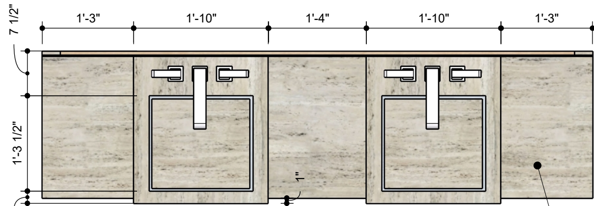
TOP VIEW
