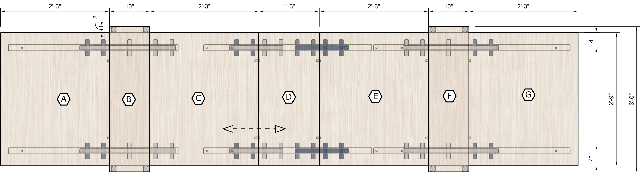
TOP VIEW Scale 1:12
