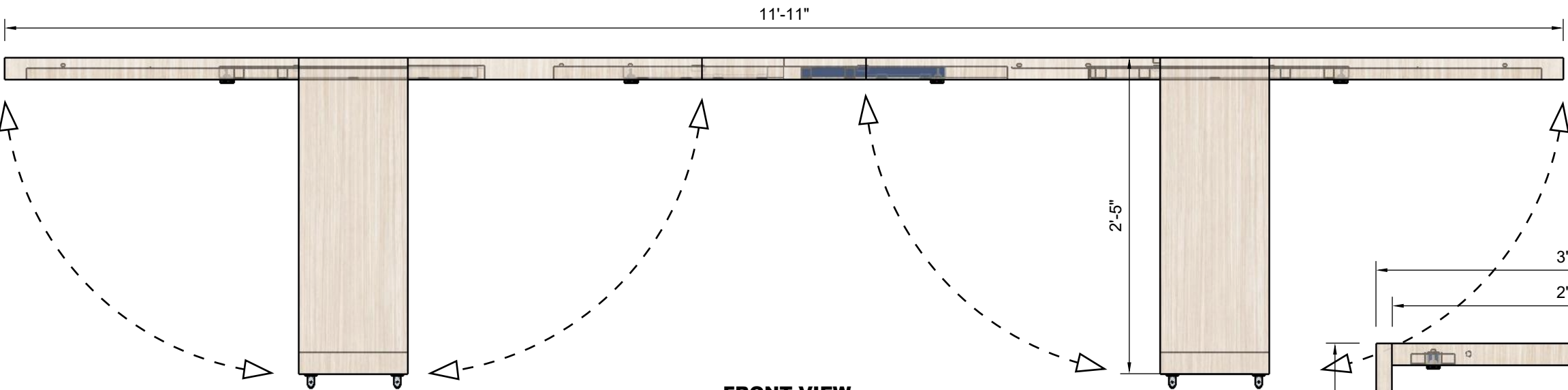
FRONT VIEW Scale 1:12
