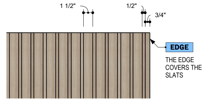
DETAIL A Scale 1:00 1.5" X .5" @ 5"
