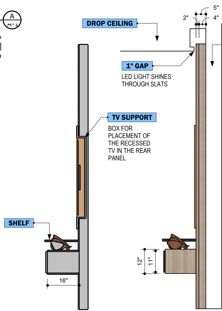
SECTION A Scale 1:00
