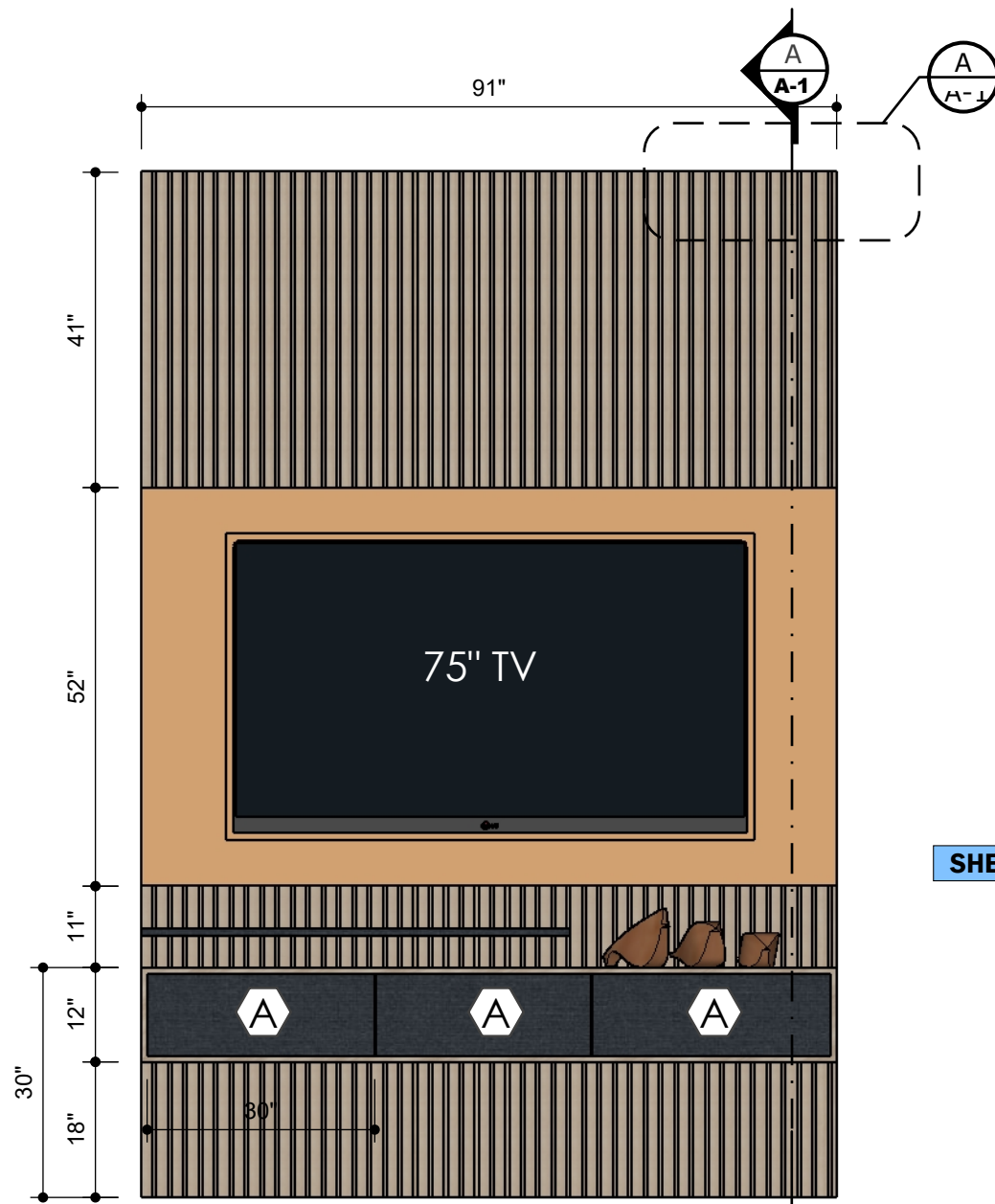
FRONT VIEW Scale 1:24
