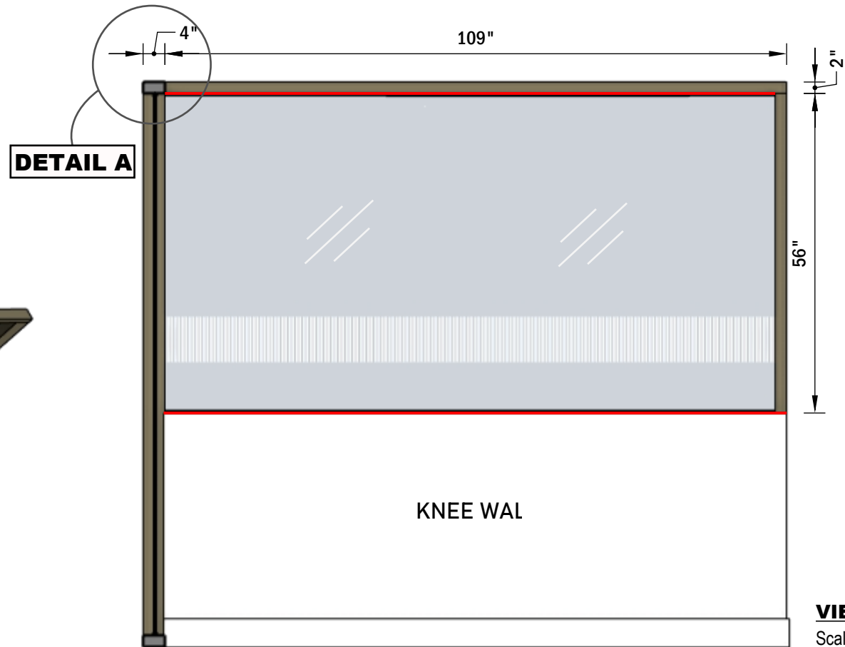
VIEW B Scale 1:24
