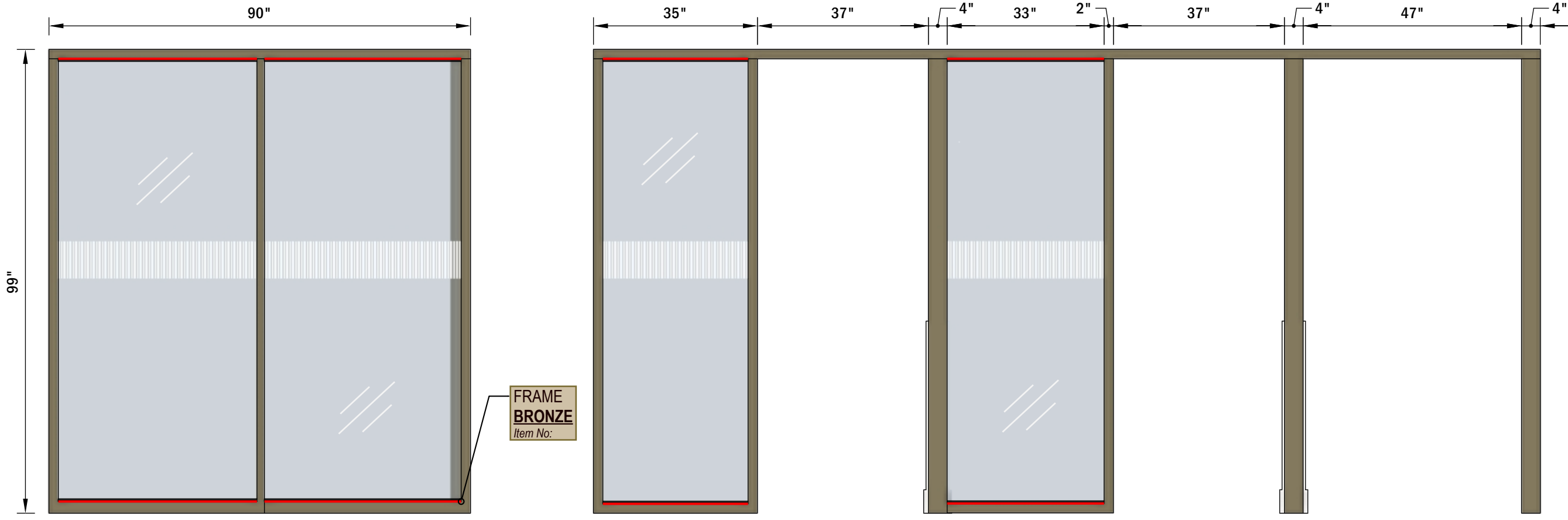
FRONT VIEW Scale 1:24
