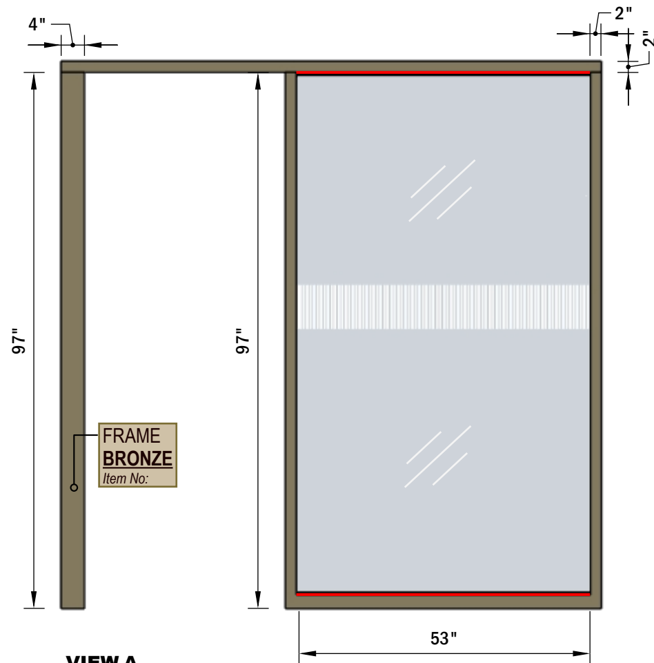
VIEW A Scale 1:24
