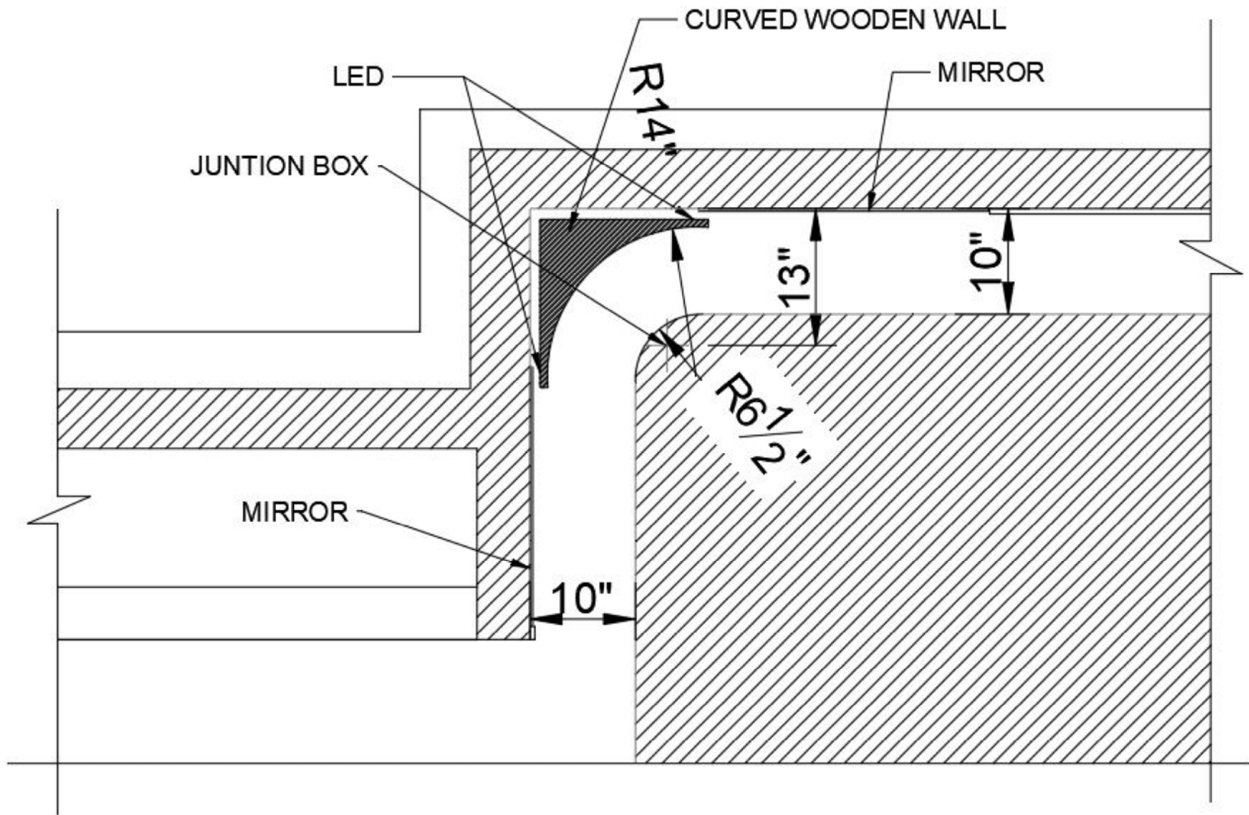
2409 FOYER CEILING TOP VIEW
