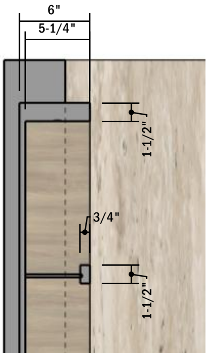
VIEW D Scale 1:8
