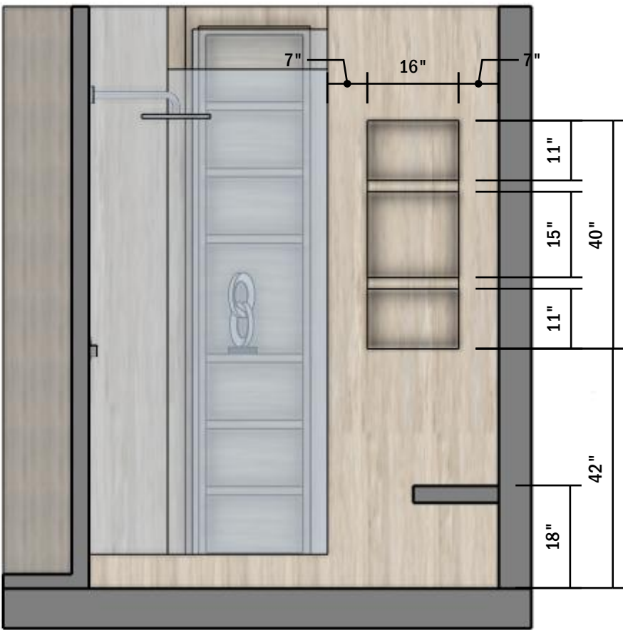
VIEW B Scale 1:00
