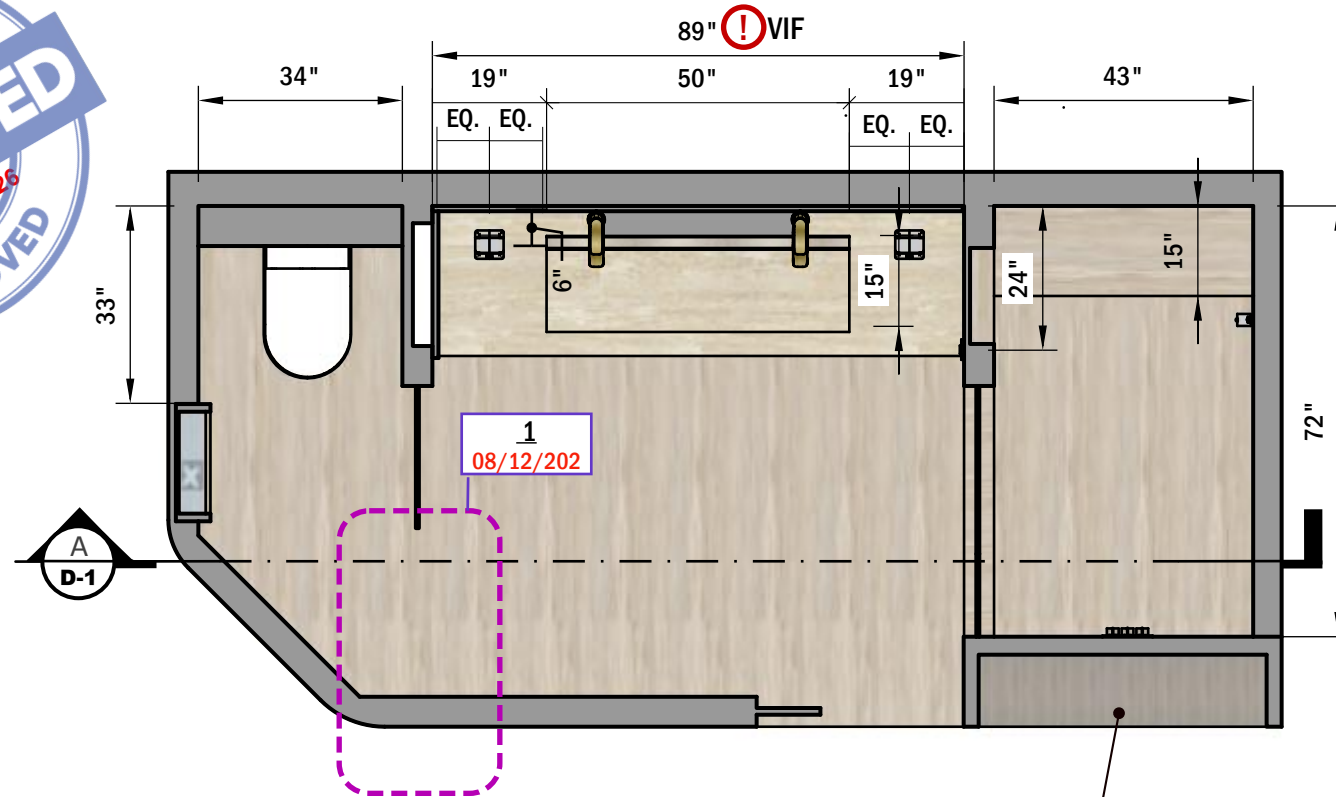
TOP VIEW Scale 1:48
