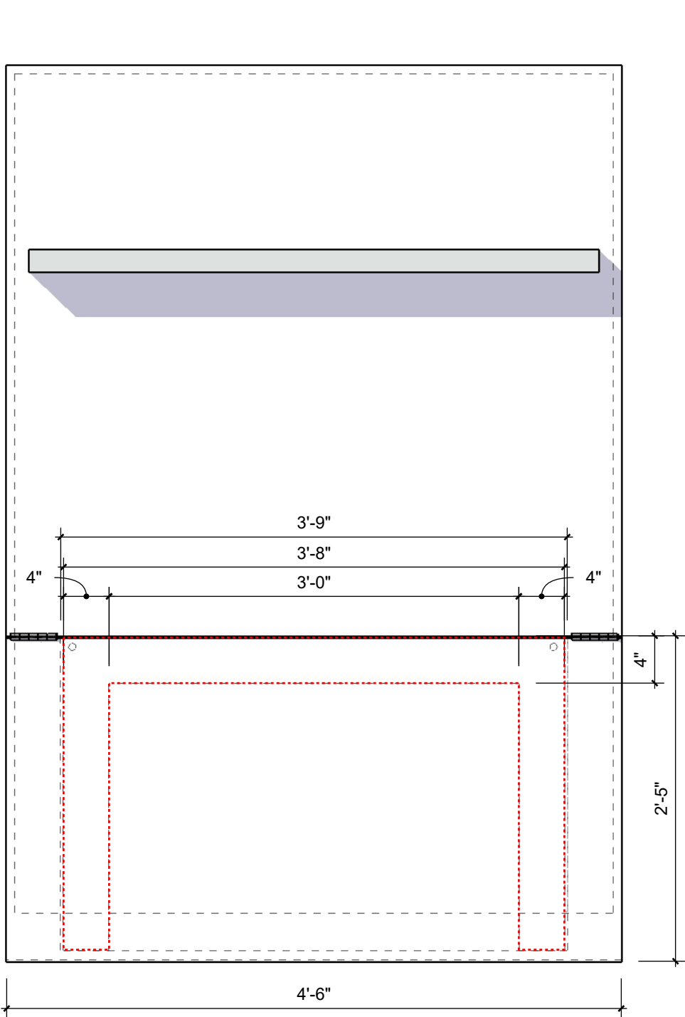
FRONT VIEW Scale 1:16
