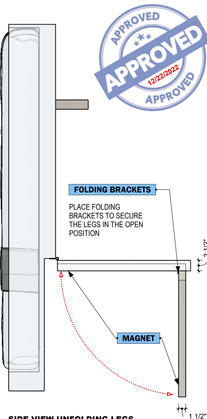
SIDE VIEW UNFOLDING LEGS Scale 1:16
