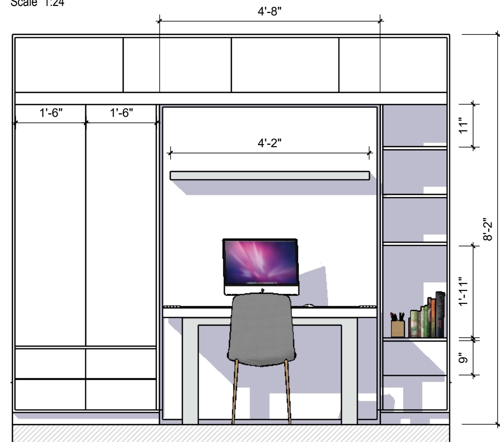
FRONT VIEW Scale 1:24
