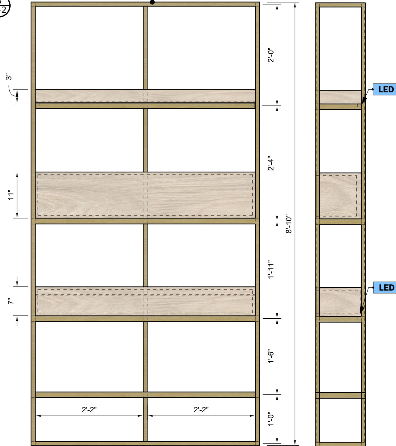
SIDE VIEW Scale 1:16
