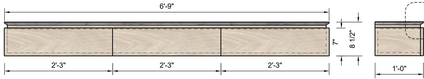
FRONT VIEW Scale 1:16
