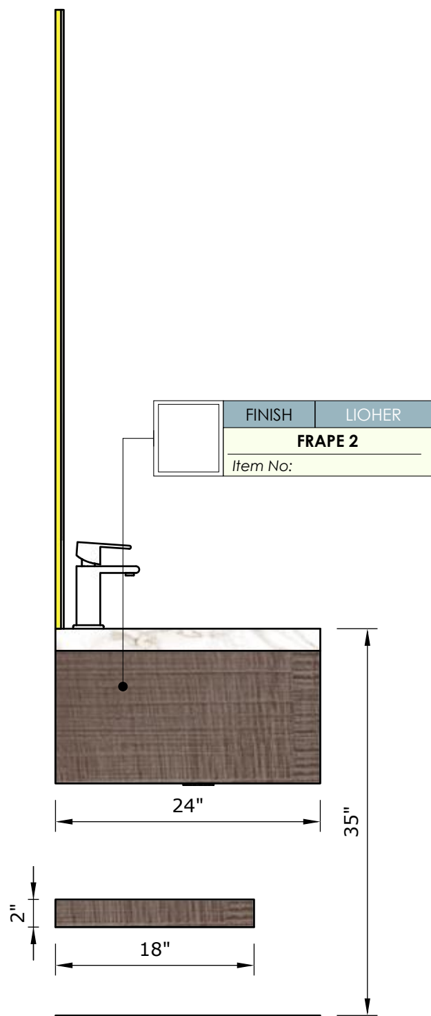
SIDE VIEW Scale 1:12
