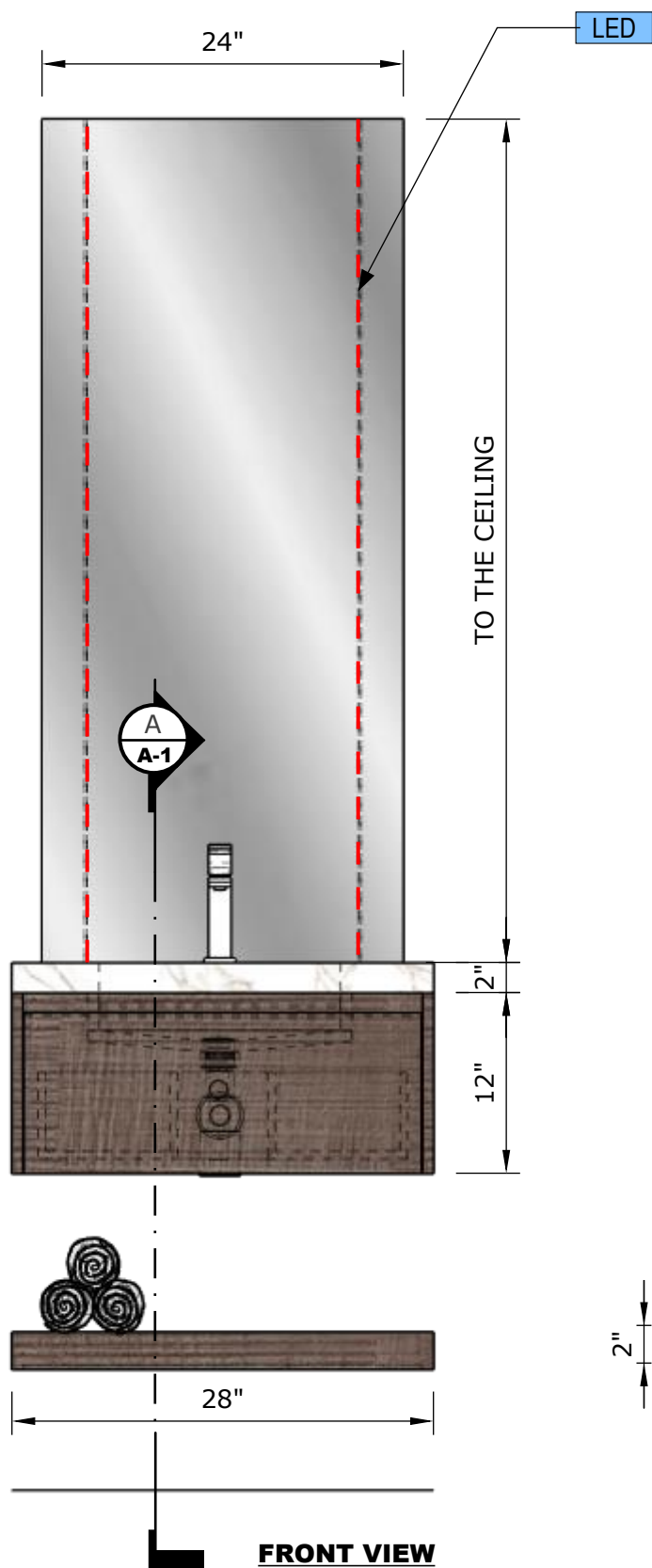
FRONT VIEW Scale 1:12
