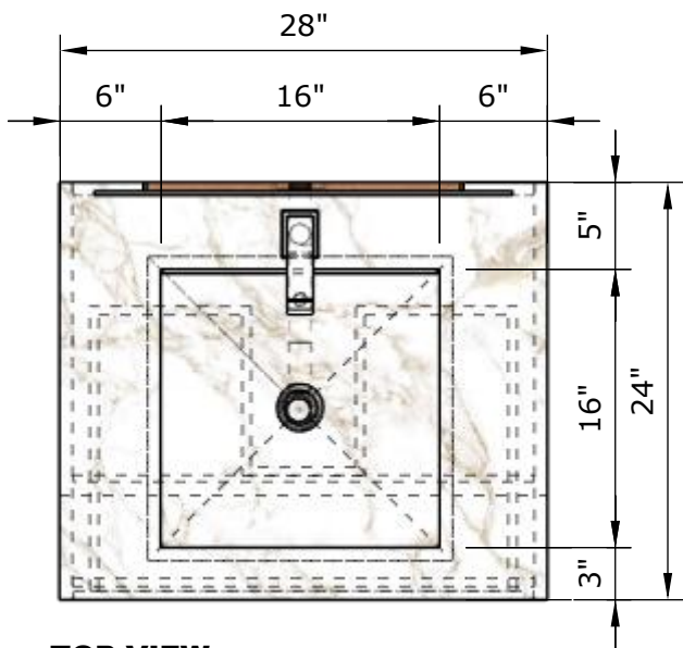
TOP VIEW Scale 1:12
