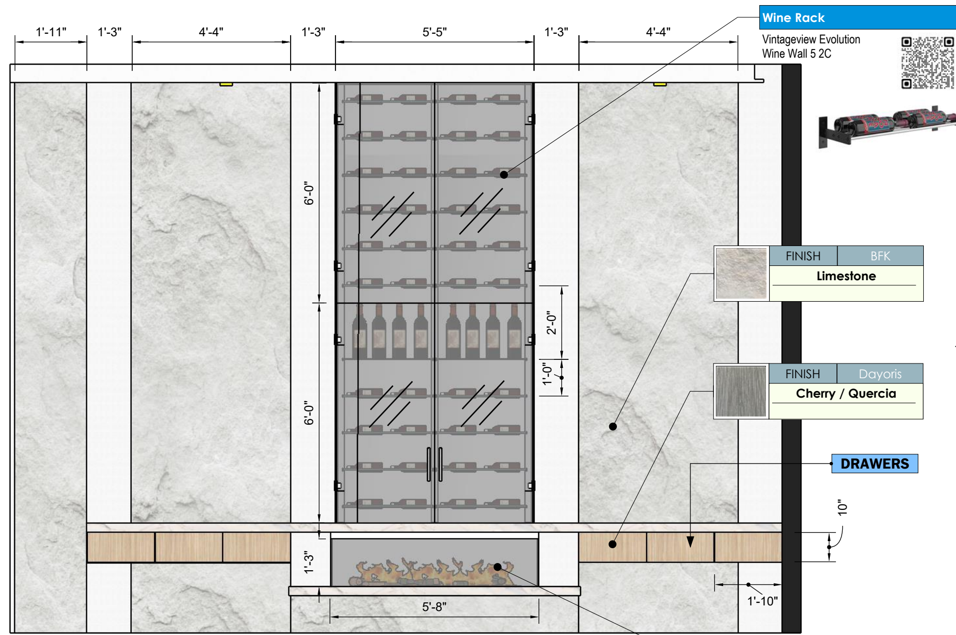
FRONT VIEW Scale 1:32
