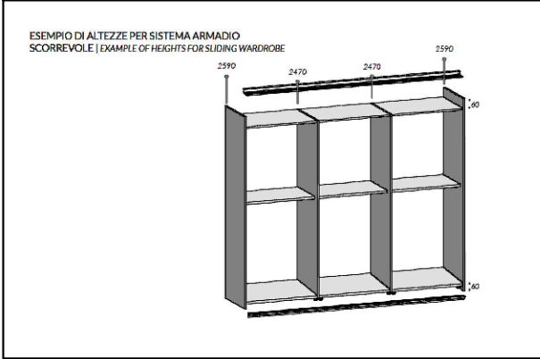
SLIDING DOORS SLIDING WARDROBE
