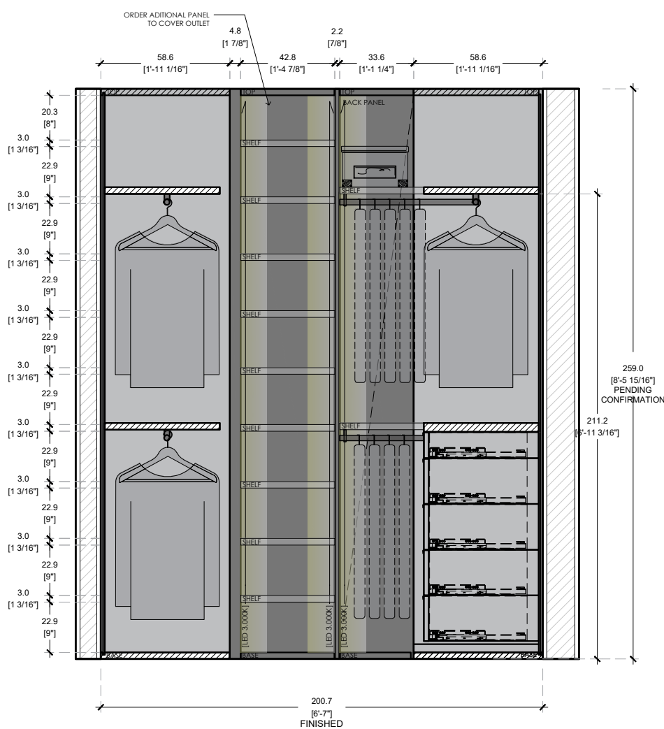
ELEVATION A SCALE 1/2"=1'-0" CONTINUUM NORTH UNIT / HIS CLOSET
