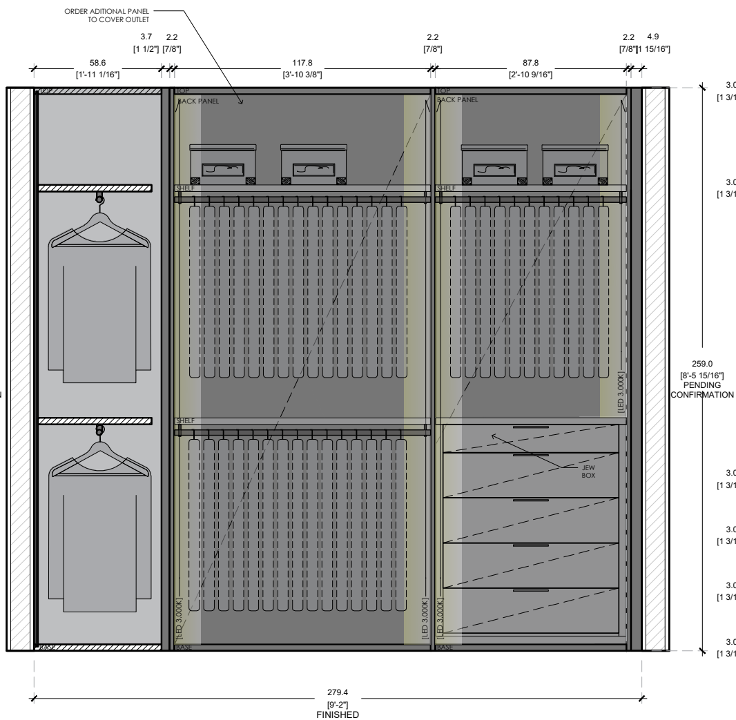
ELEVATION B SCALE 1/2"=1'-0" CONTINUUM NORTH UNIT / HIS CLOSET
