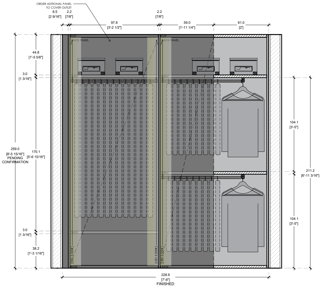
ELEVATION A PLAN SCALE 1/2"=1'-0" CONTINUUM NORTH UNIT / HER CLOSET
