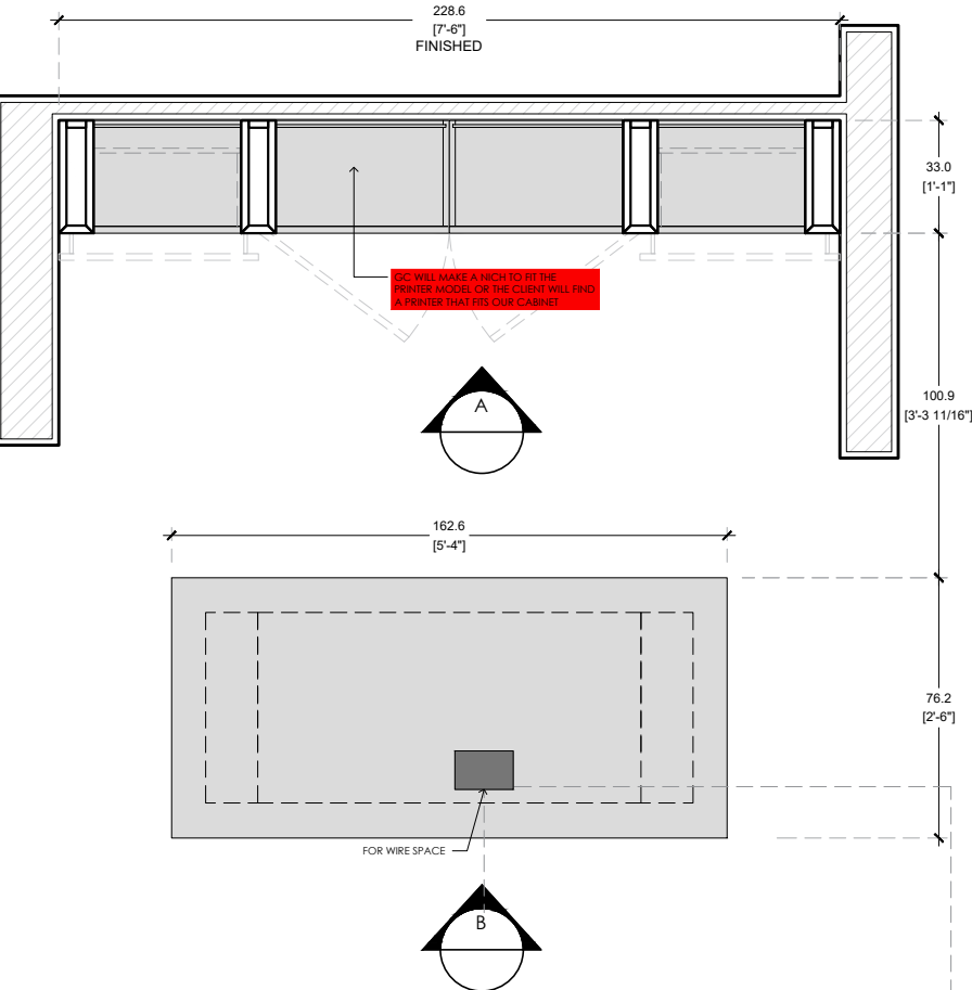
FLOOR PLAN SCALE 1/2"=1'-0" CONTINUUM NORTH UNIT /OFFICE
