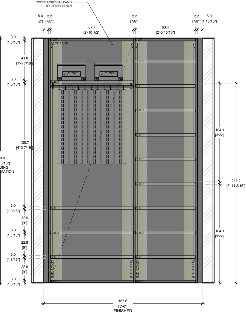
ELEVATION C SCALE 1/2"=1'-0" CONTINUUM NORTH UNIT / HIS CLOSET
