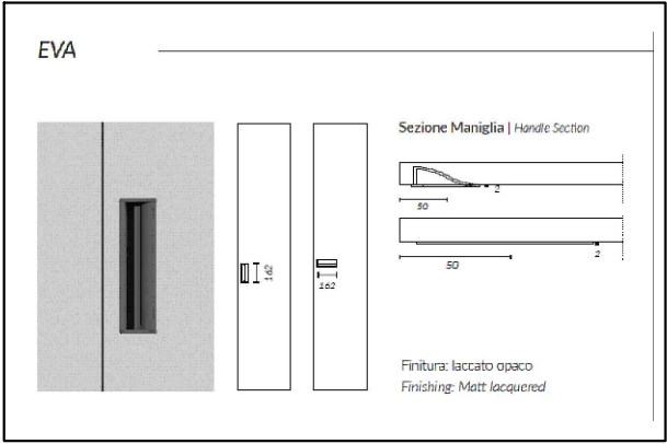
HANDLE DRAWERS EVA
