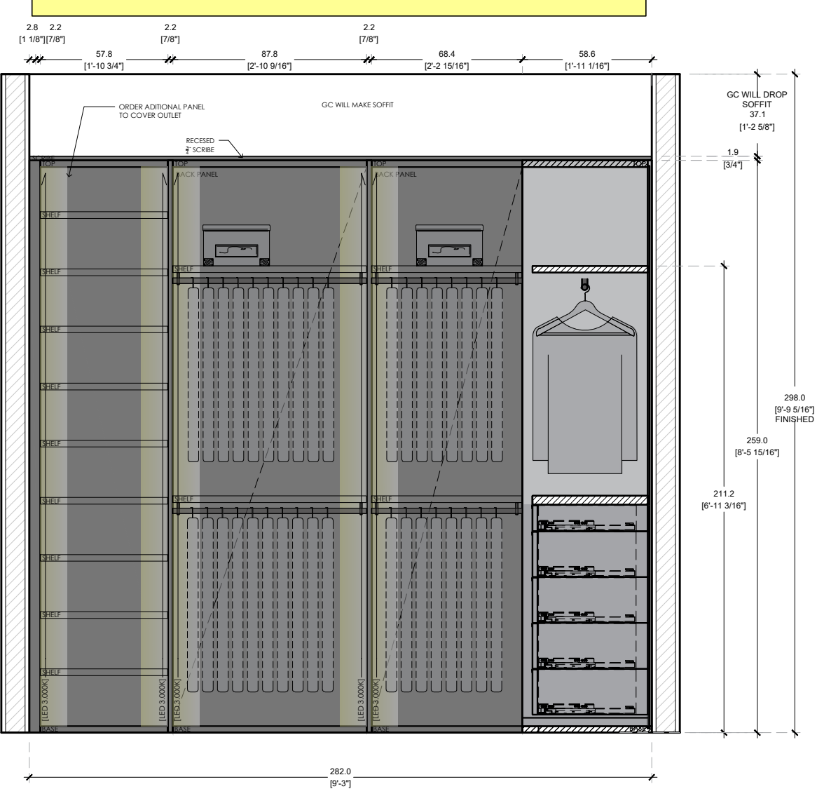
ELEVATION A SCALE 1/2"=1'-0" CONTINUUM NORTH UNIT / BEDROOM 2 CLOSET
