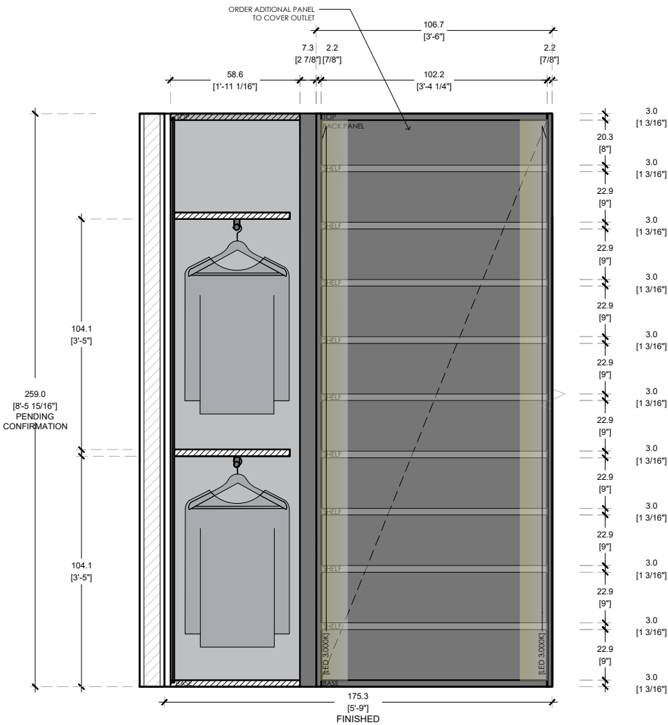
ELEVATION D SCALE 1/2"=1'-0" CONTINUUM NORTH UNIT / HER CLOSET
