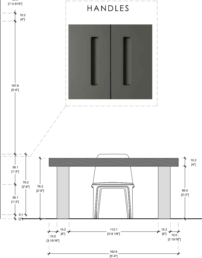
ELEVATION B SCALE 1/2"=1'-0" CONTINUUM NORTH UNIT /OFFICE
