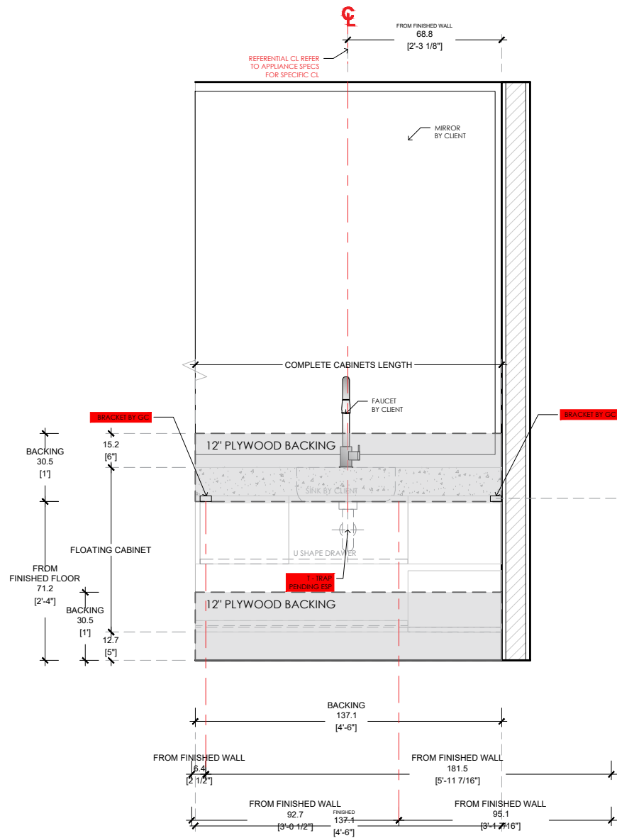
ELEVATION A SCALE 1/2"=1'-0" CONTINUUM NORTH UNIT 2901 / BEDROOM 3 CLOSET
