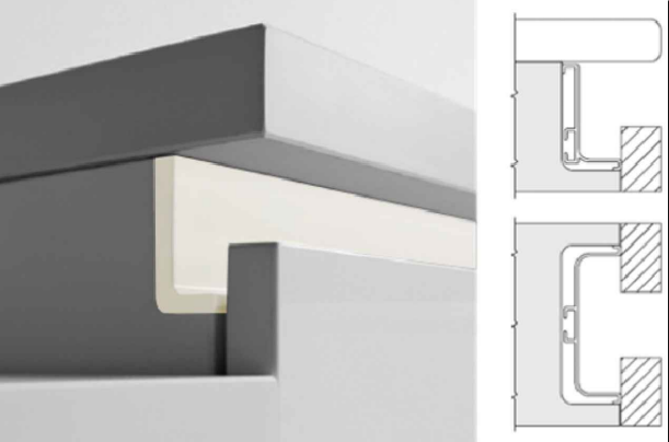
BASE CABINETS INTEGRATED GOLA - MATCH FINISH 1
