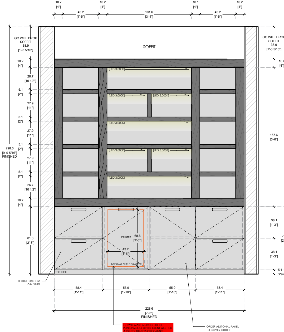
ELEVATION A SCALE 1/2"=1'-0" CONTINUUM NORTH UNIT /OFFICE
