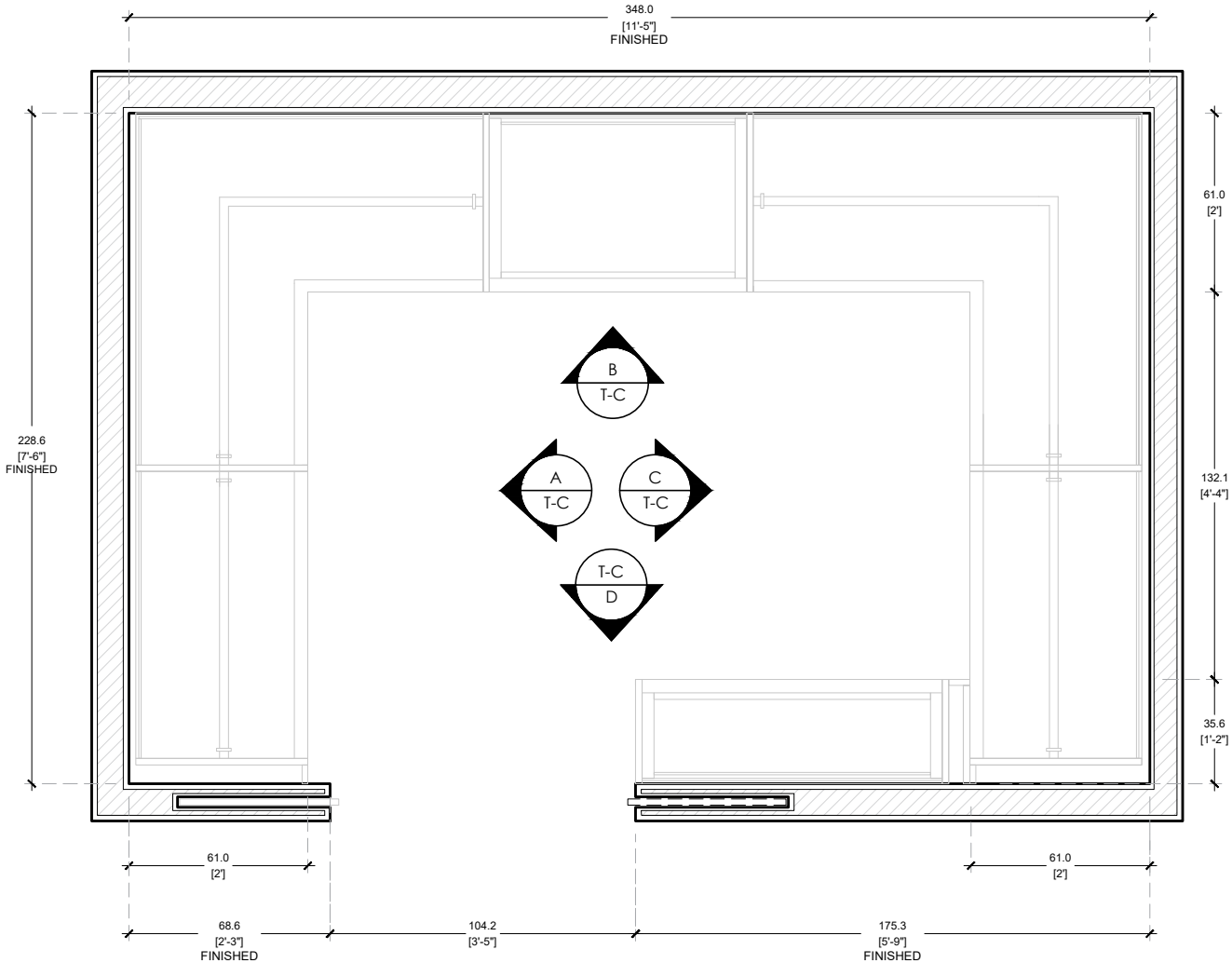
FLOOR PLAN SCALE 1/2"=1'-0" CONTINUUM NORTH UNIT 2901 / HER CLOSET
