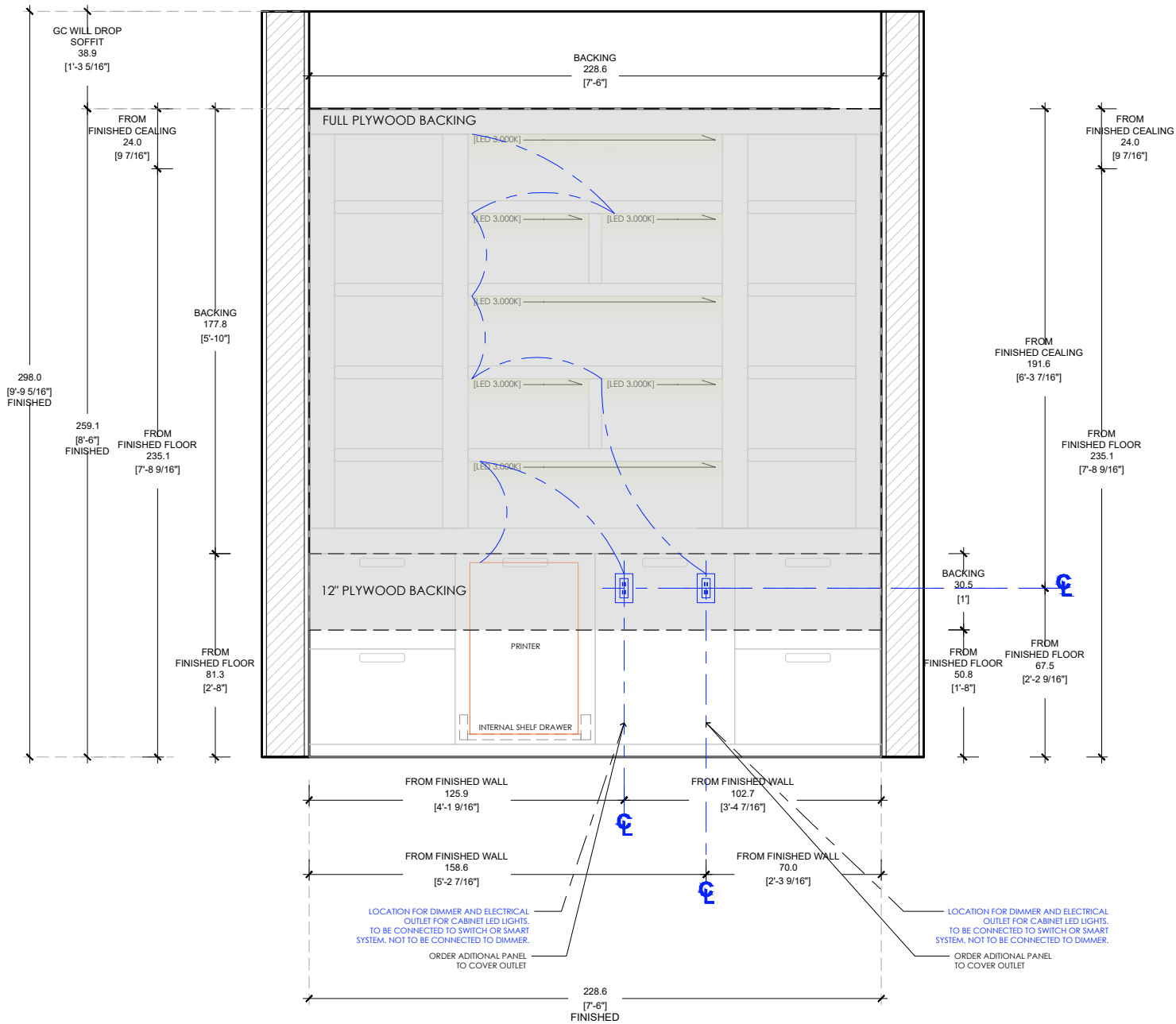
ELEVATION A SCALE 1/2"=1'-0" CONTINUUM NORTH UNIT 2901 / OFFICE
