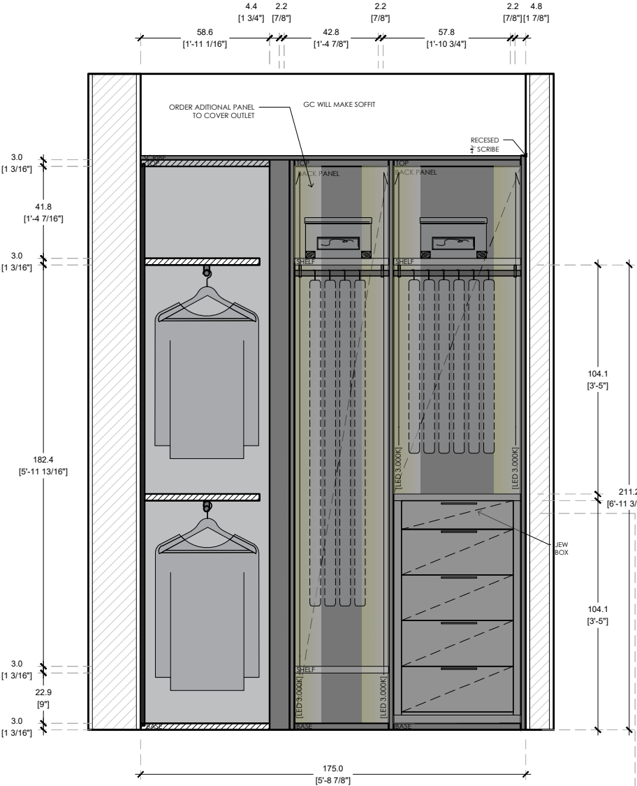
ELEVATION B SCALE 1/2"=1'-0" CONTINUUM NORTH UNIT / BEDROOM 2 CLOSET
