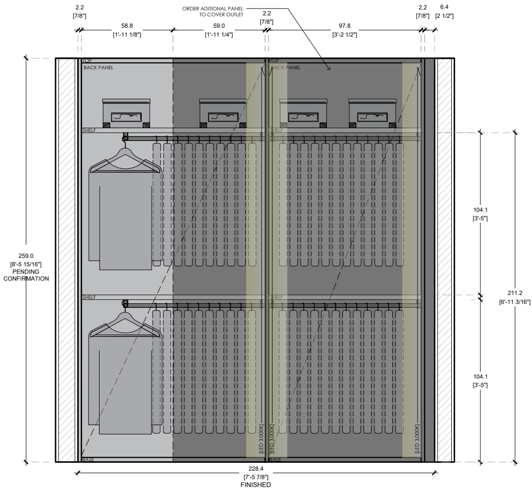
ELEVATION C SCALE 1/2"=1'-0" CONTINUUM NORTH UNIT / HER CLOSET
