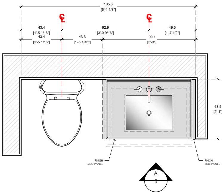
FLOOR PLAN SCALE 1/2"=1'-0" CONTINUUM NORTH UNIT / BEDROOM 3 BATHROOM
