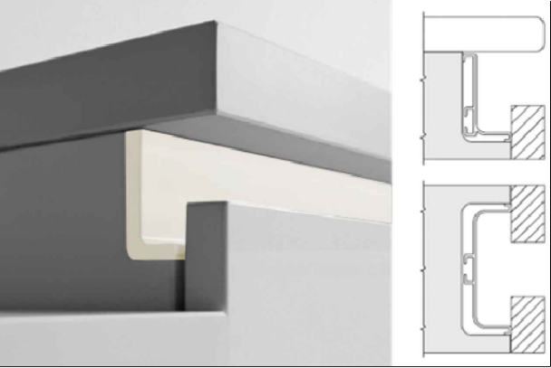
BASE CABINETS INTEGRATED GOLA - MATCH FINISH 2
