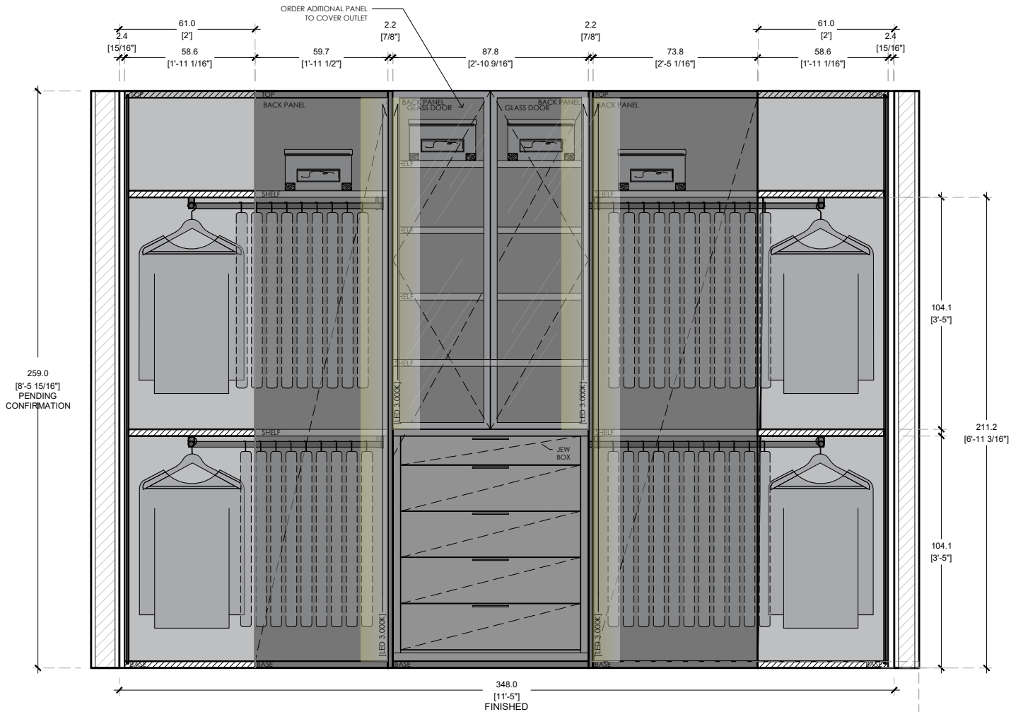
ELEVATION B SCALE 1/2"=1'-0" CONTINUUM NORTH UNIT / HER CLOSET
