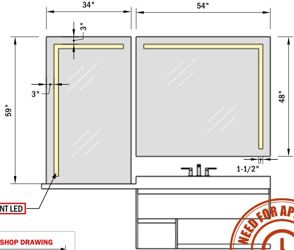
MASTER HER MIRRORS Scale 1:24
