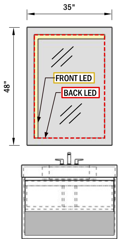
MIRROR No 2 Scale 1:24
