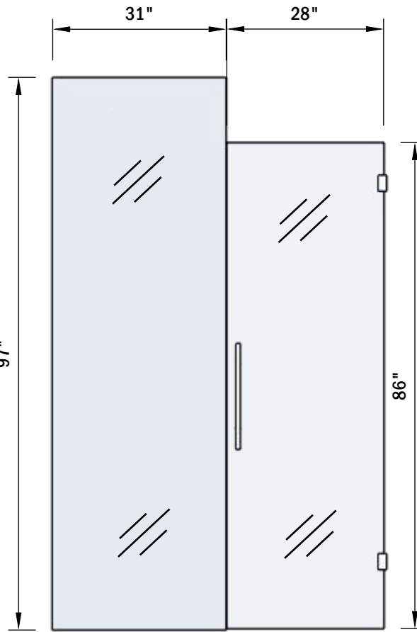
SHOWER ENCLOSURE No 2 Scale 1:24
