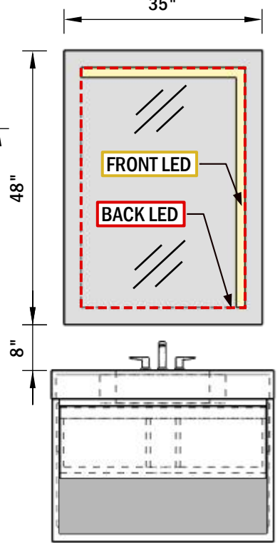
MIRROR No 3 Scale 1:24
