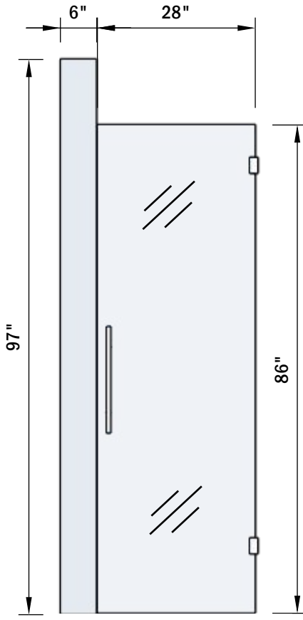
SHOWER ENCLOSURE No 3 Scale 1:24
