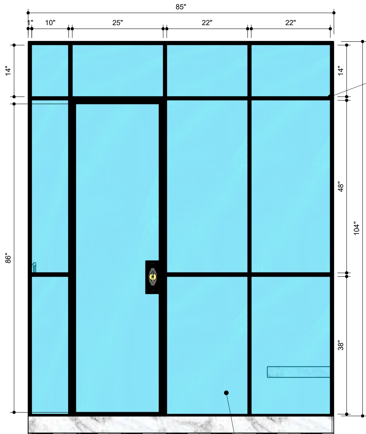
FRONT VIEW Scale 1:16
