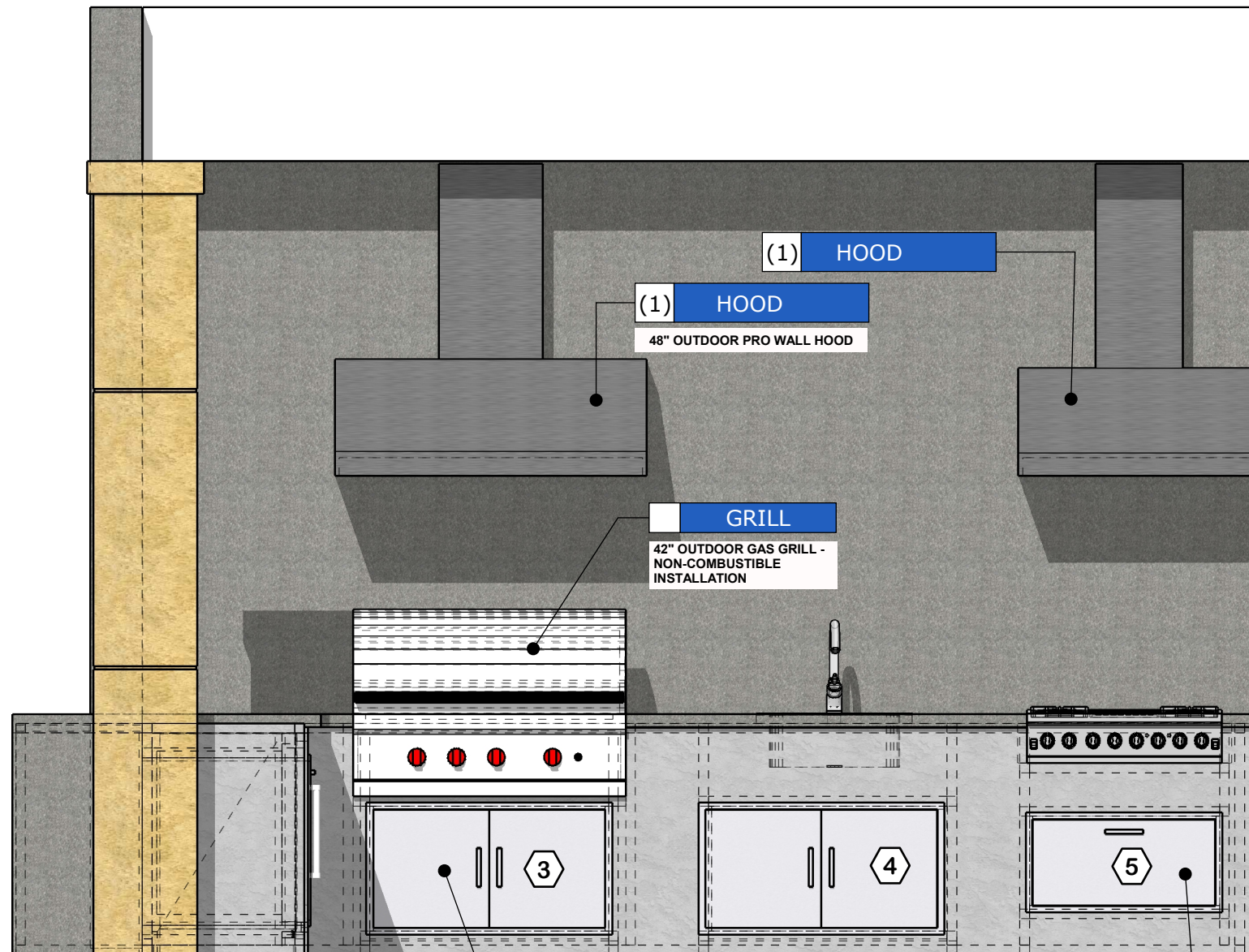
FRONT VIEW Scale 1:24
