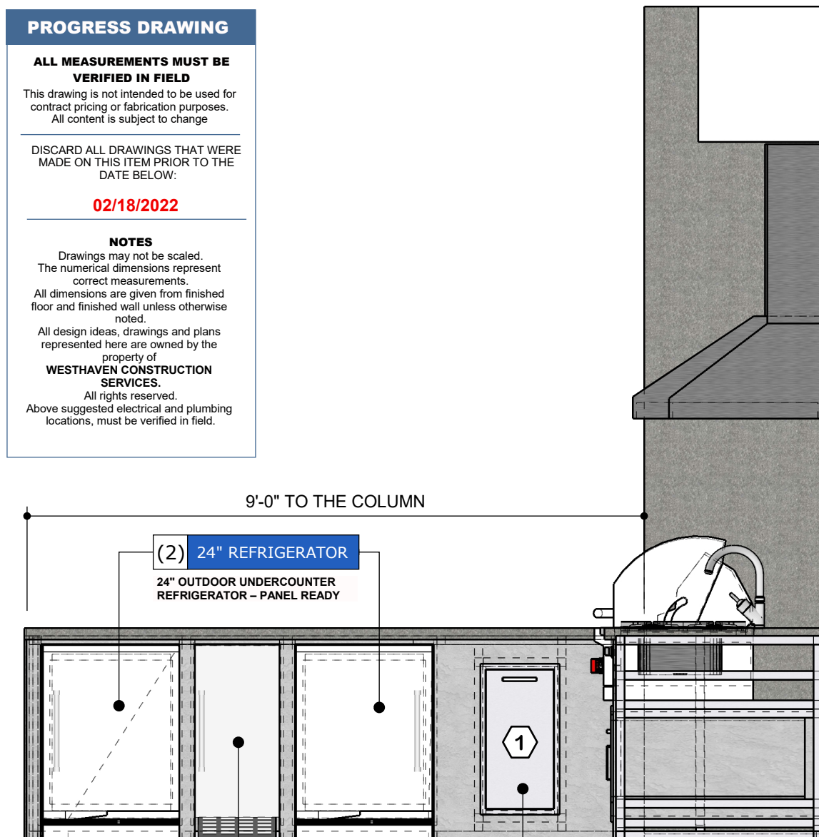
SIDE VIEW Scale 1:24
