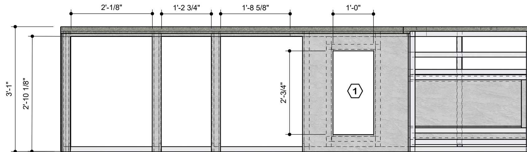
VIEW 1 Scale 1:24
