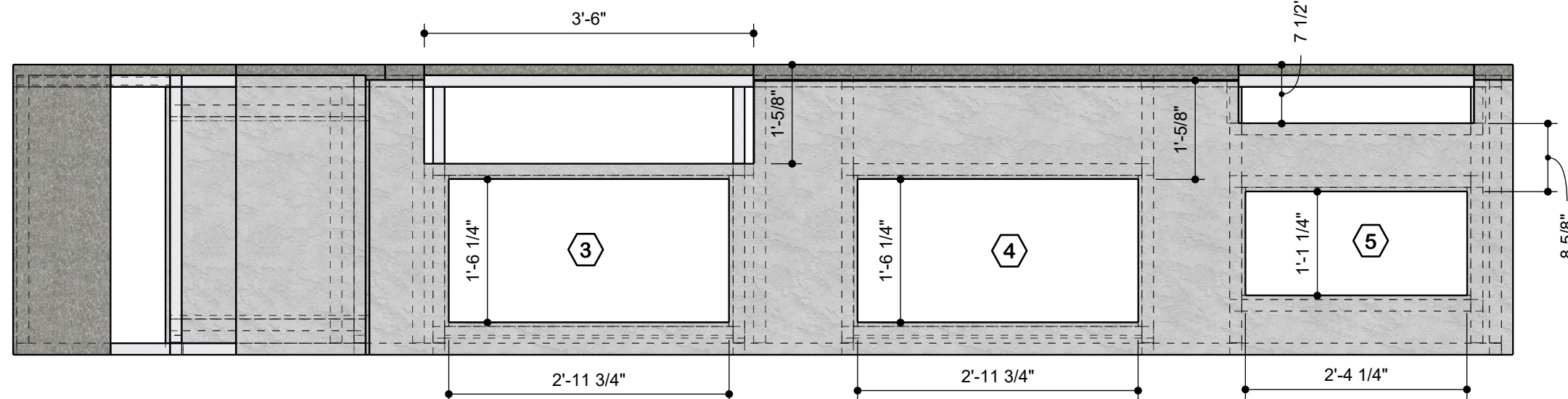
VIEW 2 Scale 1:24
