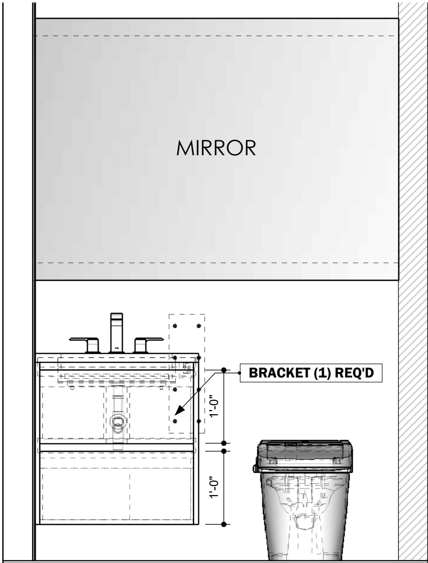
FRONT VIEW
