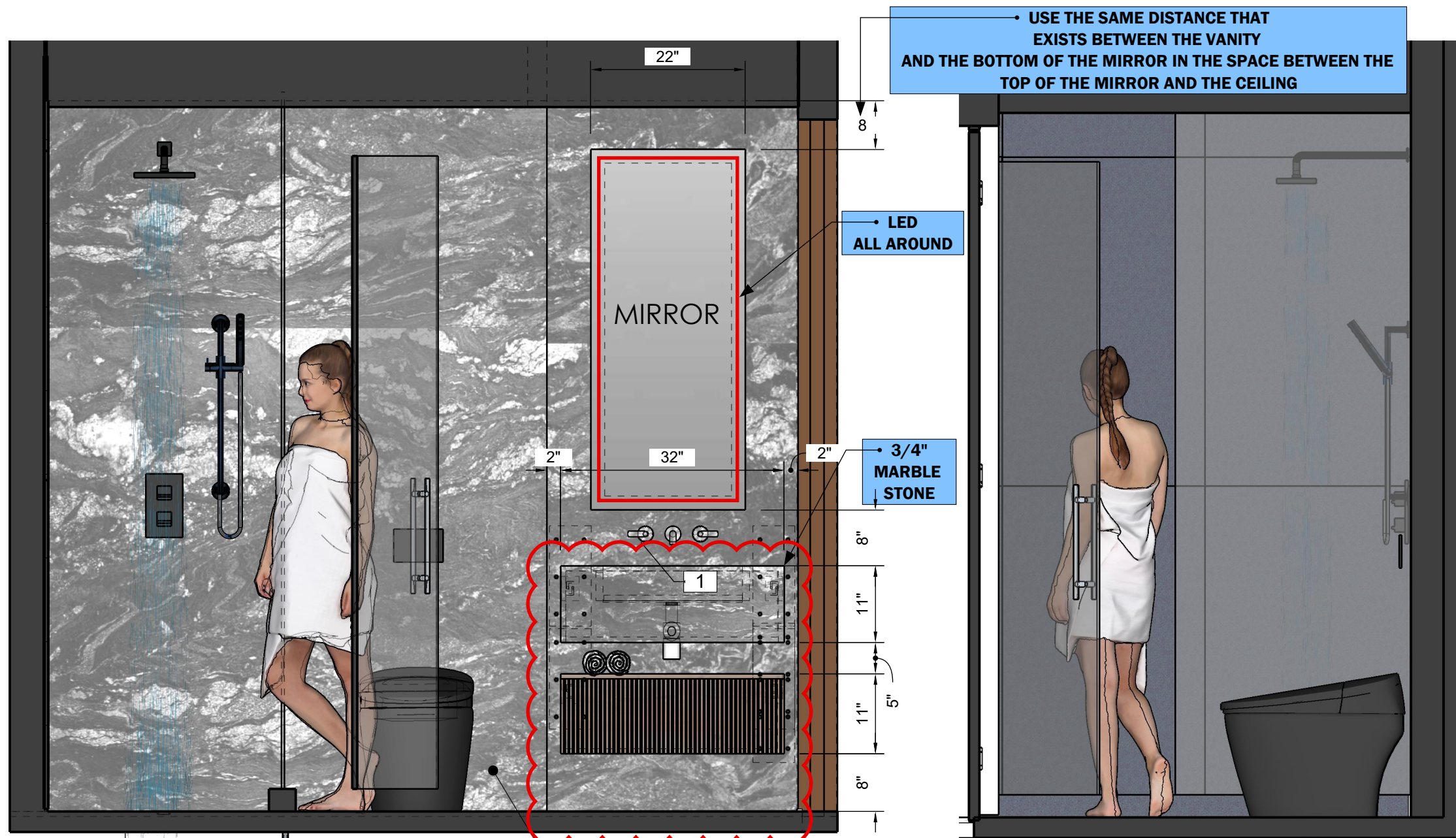
SECTION A Scale 1:00
