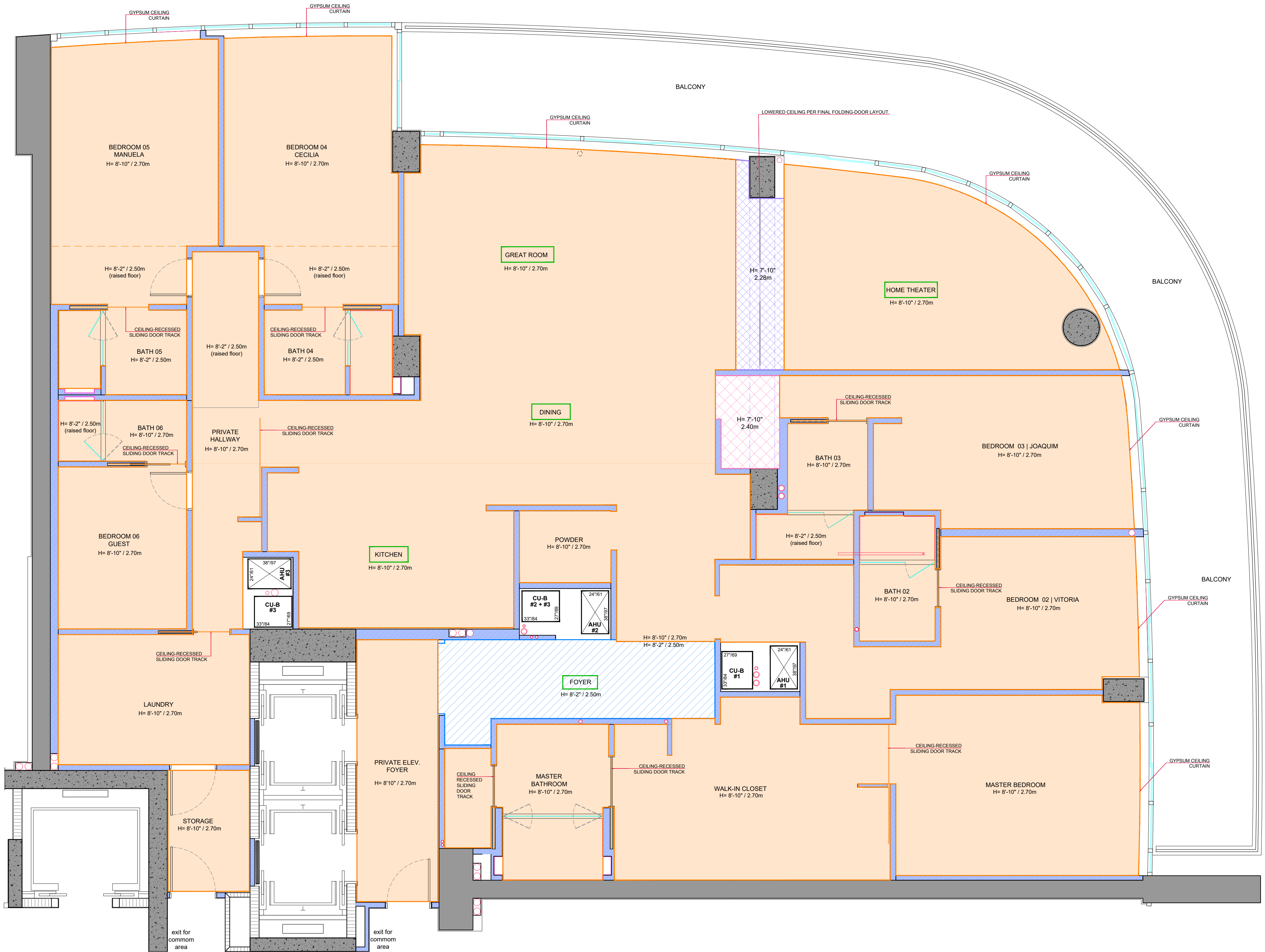
CEILING PLAN scale 1/4" = 1'-0" scale 1:50
