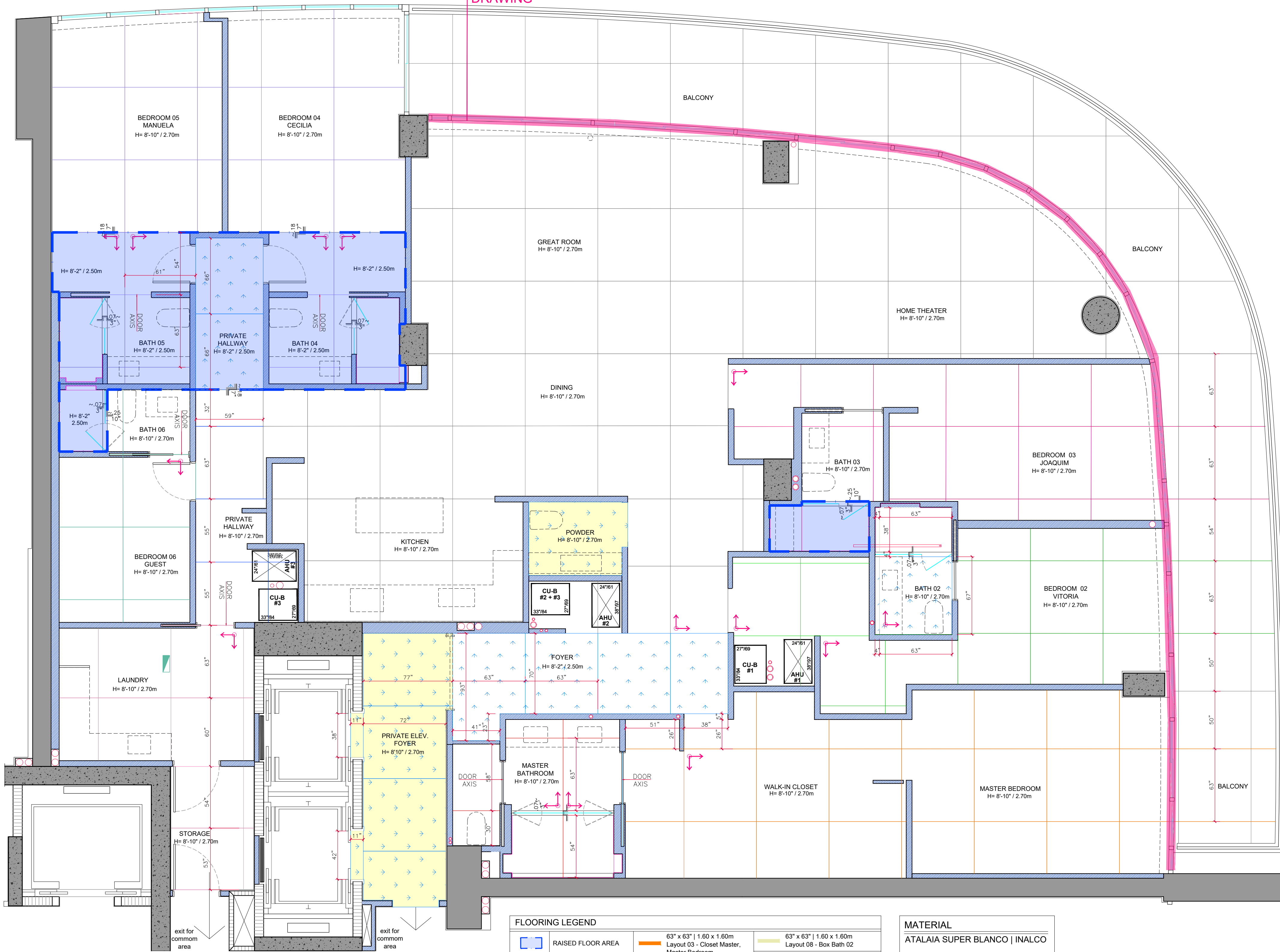
FLOORING PLAN scale 1/4" = 1'-0" measurements in inches
