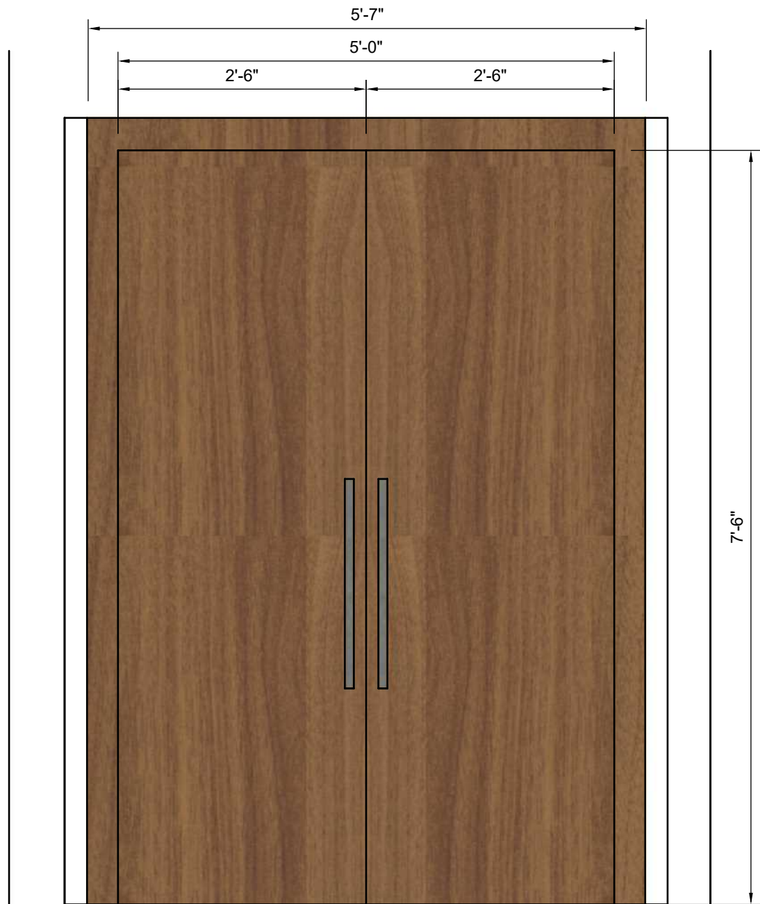
FRONT VIEW Scale 1:16
