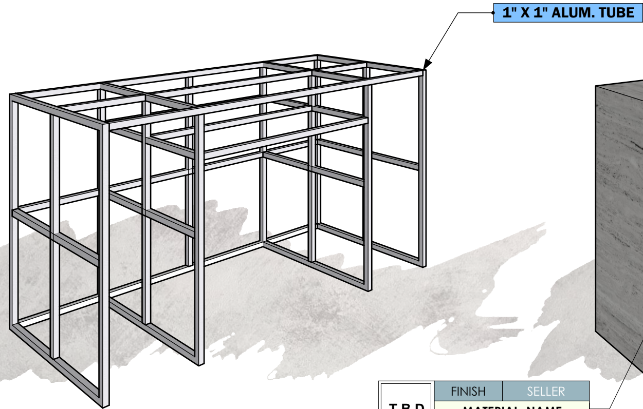
STRUCTURE Not Scaled
