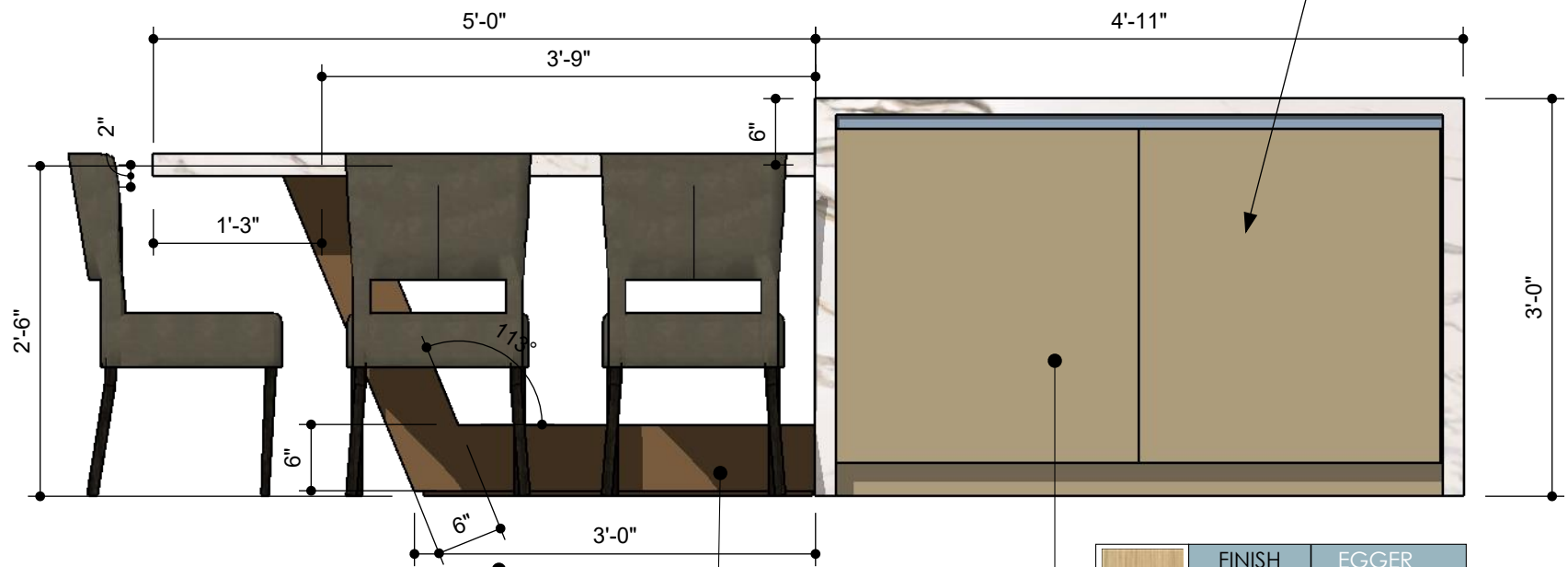
FRONT VIEW
