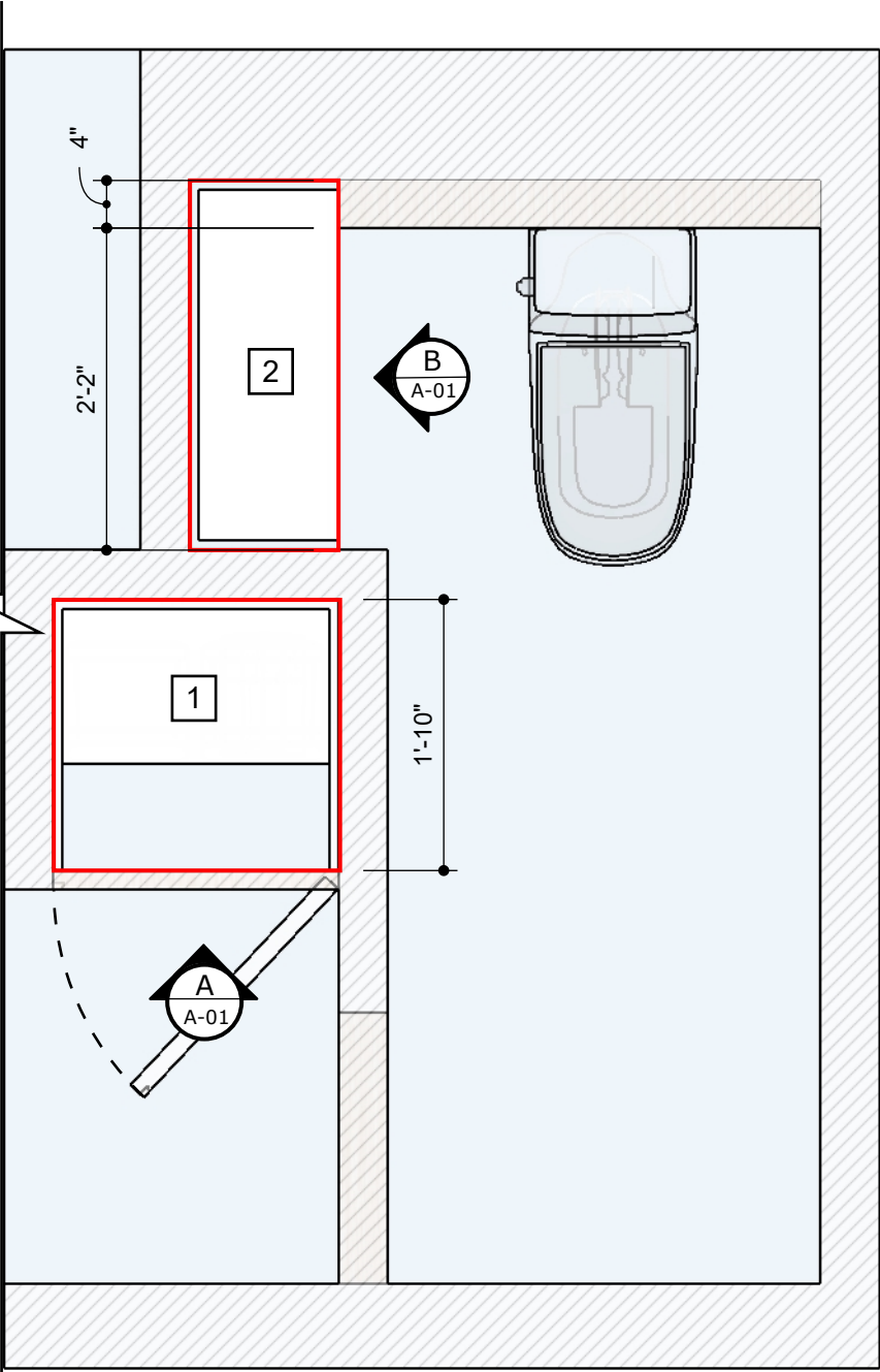
TOP VIEW Scale 1:16
