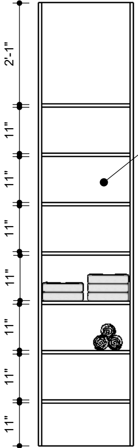
VIEW A Scale 1:00
