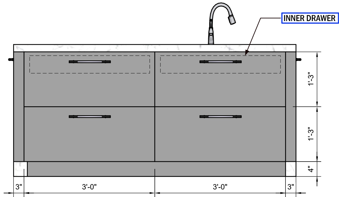
FRONT VIEW
