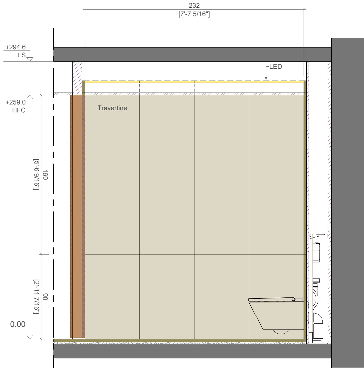
ELEVATION AA
