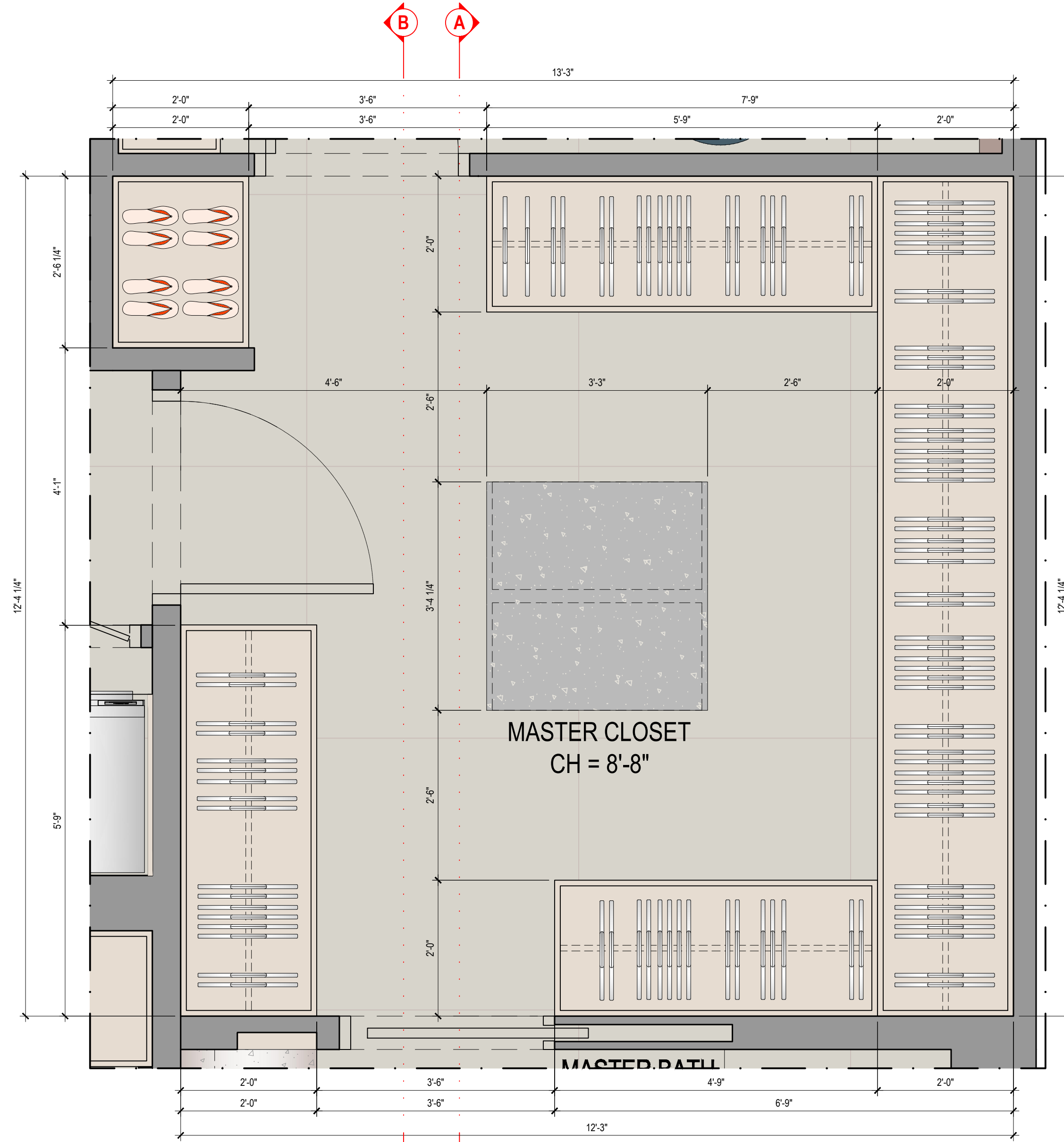
MASTER CLOSET - FLOOR PLAN SCALE: 3/4" = 1' 0"
