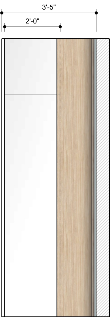
VIEW B Scale 1:24
