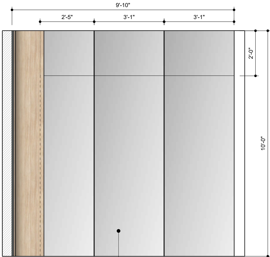
VIEW A Scale 1:24
