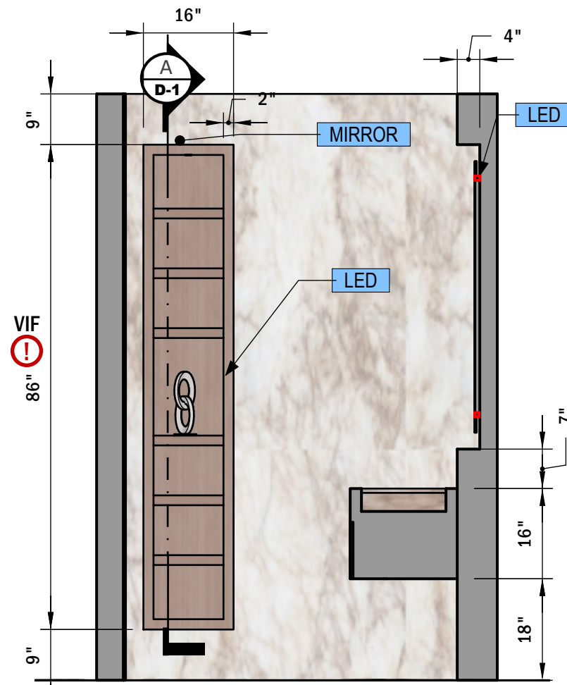
SIDE VIEW Scale 1:24
