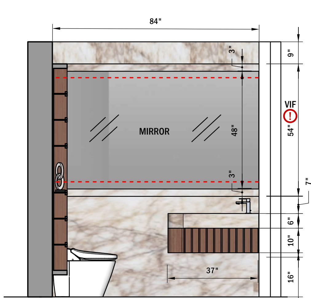
FRONT VIEW Scale 1:24
