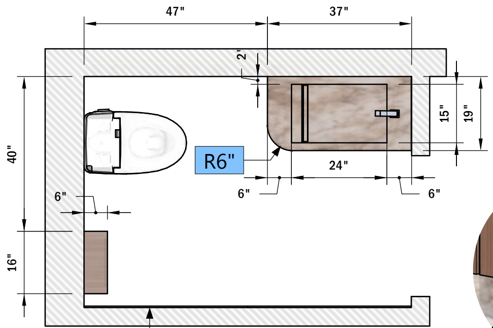
TOP VIEW Scale 1:24
