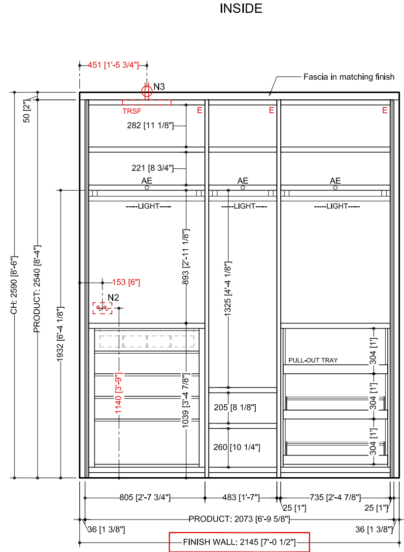
BEDROOM 3 - CLOSET ELEVATION
