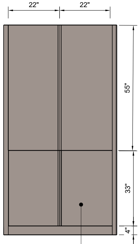
FRONT VIEW Scale 1:24
