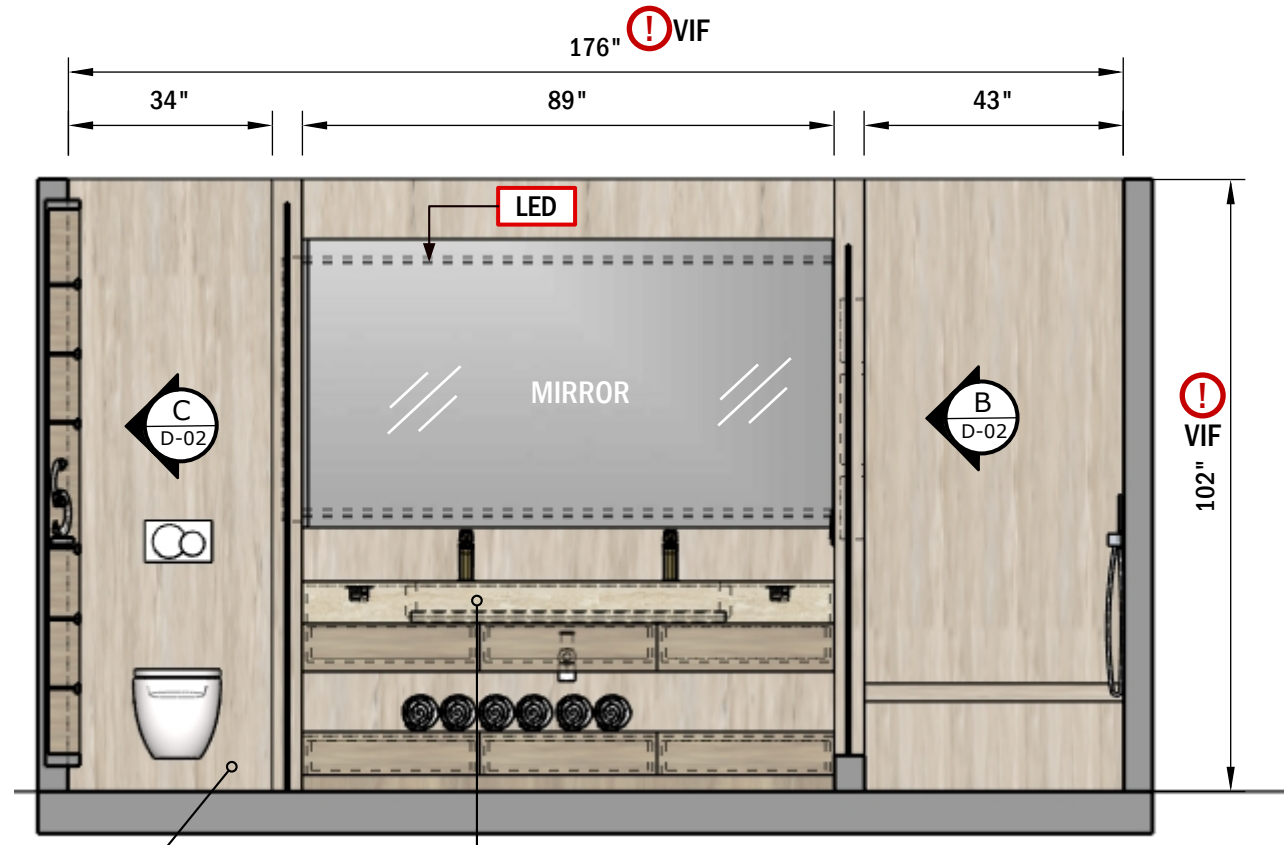
SECTION A Scale 1:00
