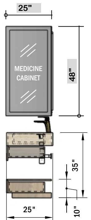
SIDE VIEW Scale 1:32
