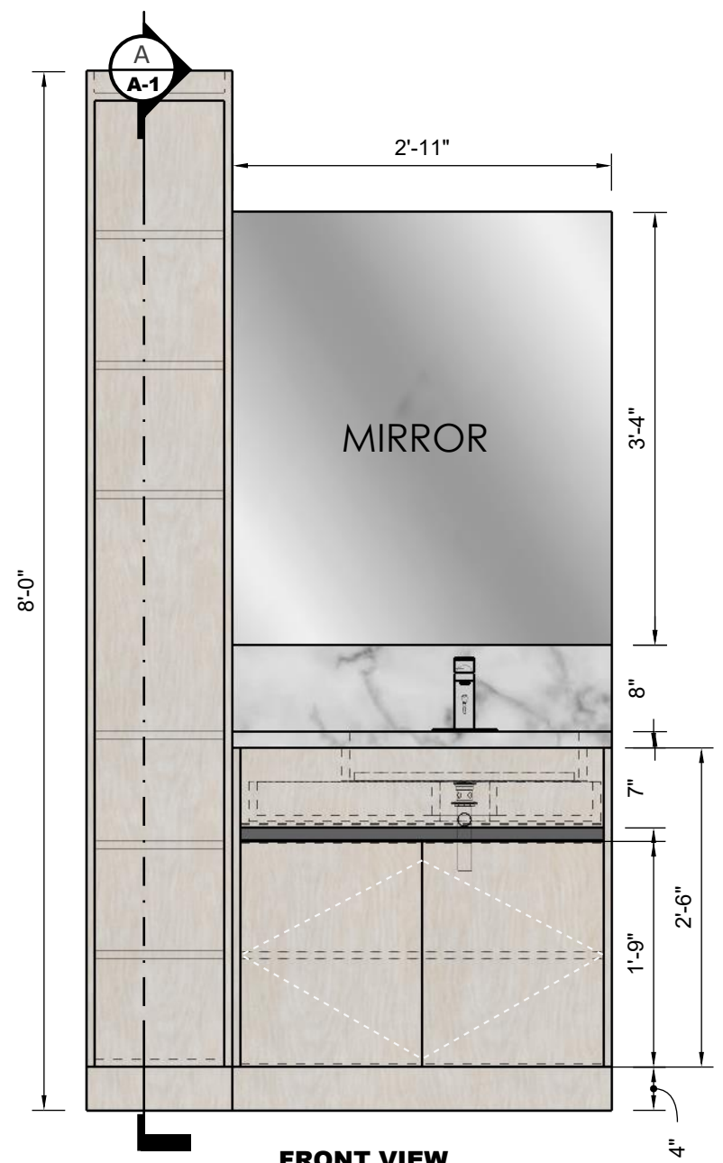
FRONT VIEW Scale 1:16
