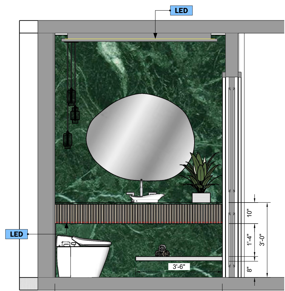
SECTION A Scale 1:00
