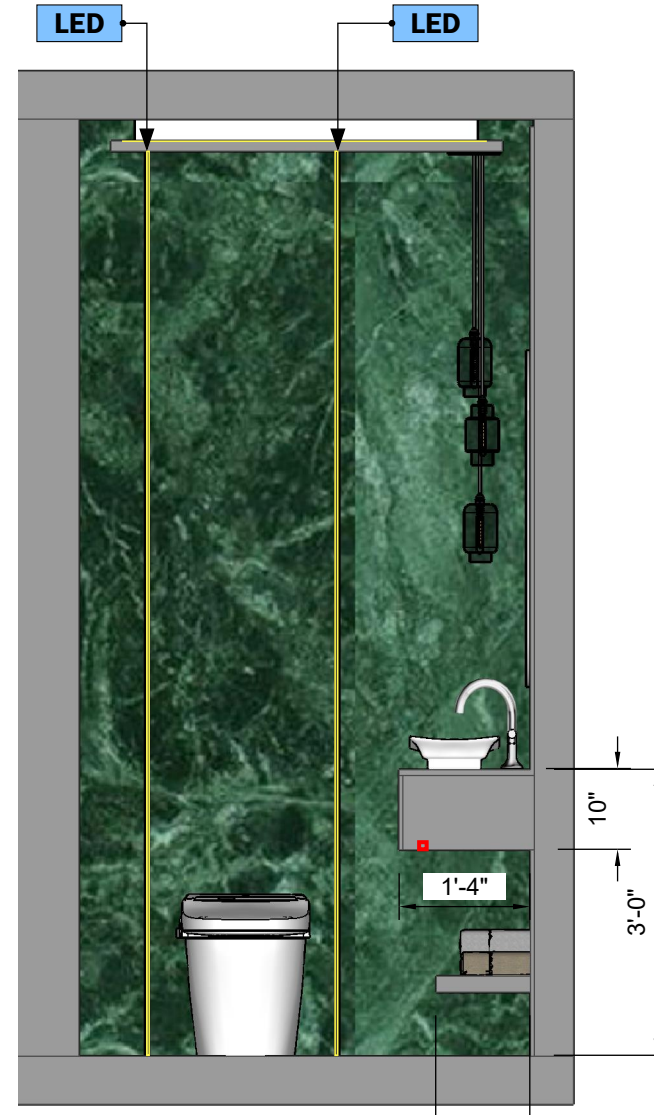
SECTION B Scale 1:00
