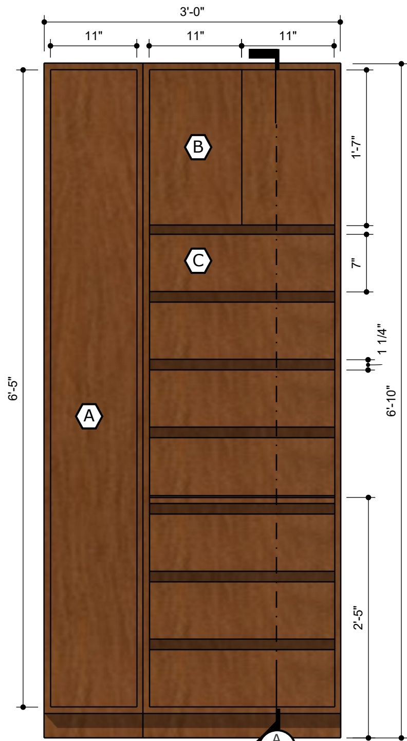
FRONT VIEW
