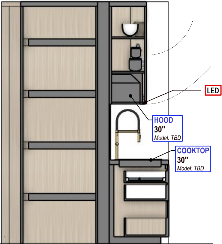
SECTION C Scale 1:24
